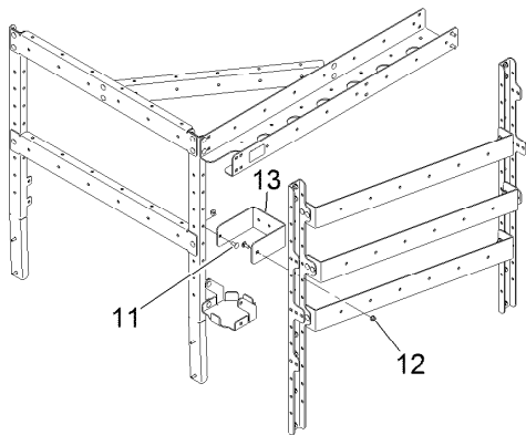
CUP CUTTER BRACKET INSTALLATION
