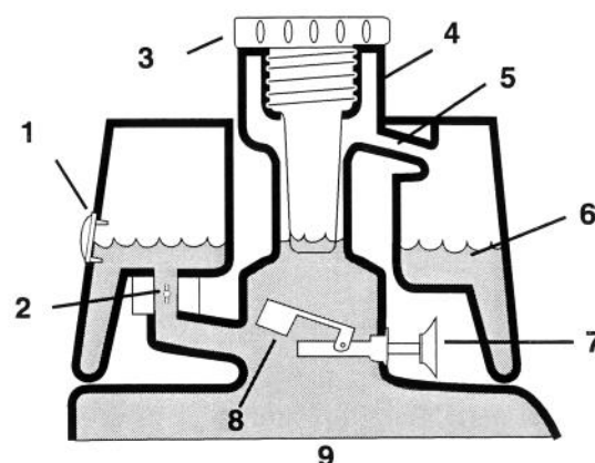
Figure 9 BEFORE START (cold oil)
