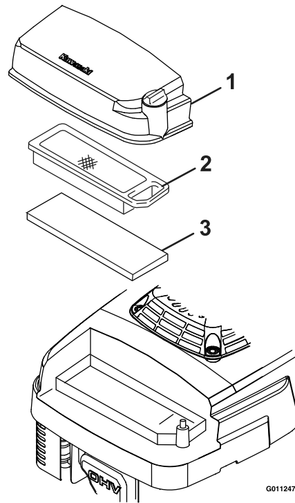
Figure 24 S-Series Units
