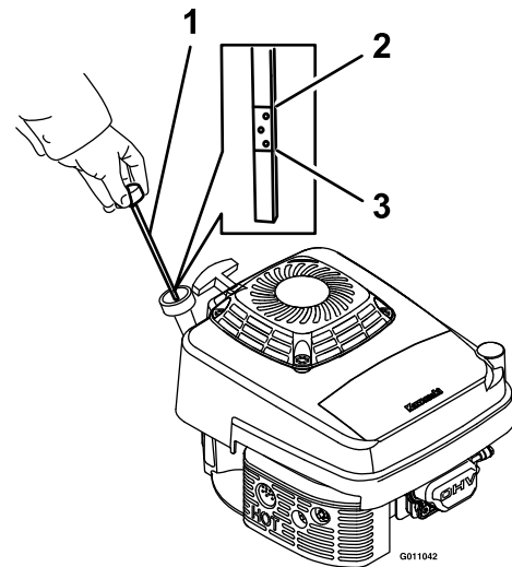
Figure 17 Kawasaki Engine
