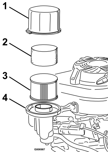
Figure 23 X-Series Units
