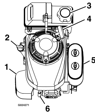
Figure 8 Honda unit
