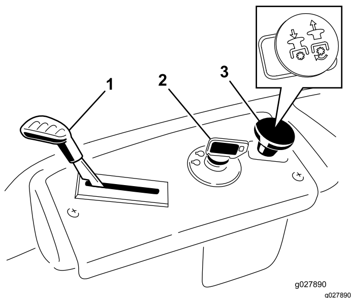
Figure 4 Control Panel
