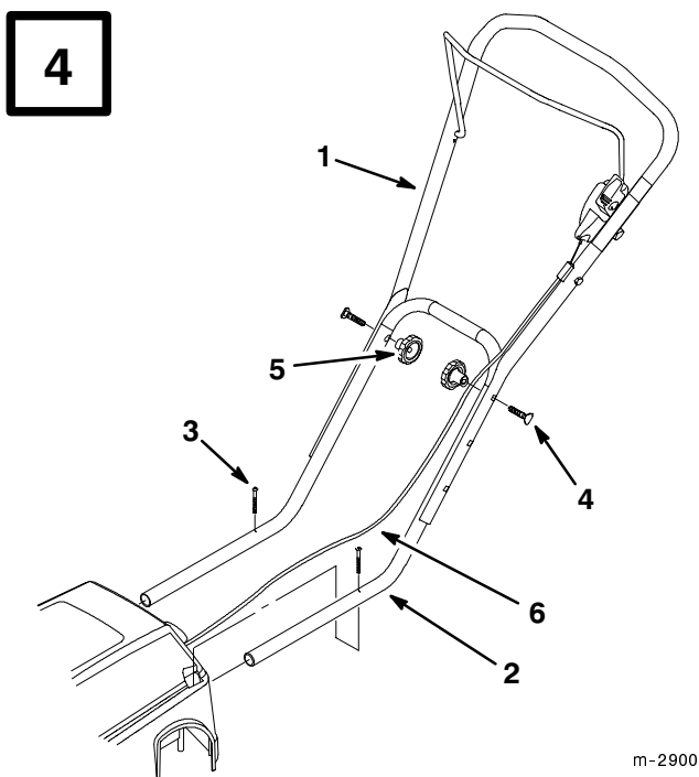
1. Upper handle 2. Lower handle 3. Screw (2) 4. Bolt (2) 5. Knob (2) 6. Control cable
