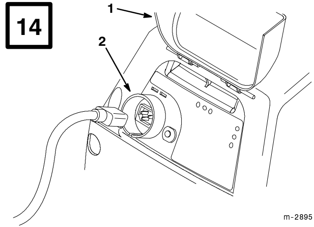
1. Rain shield 2. Plug receptacle
