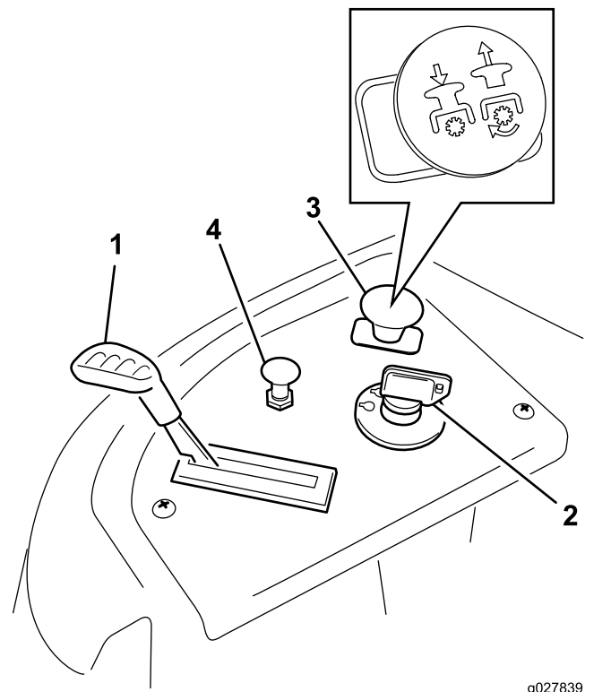
Figure 5 Control Panel
