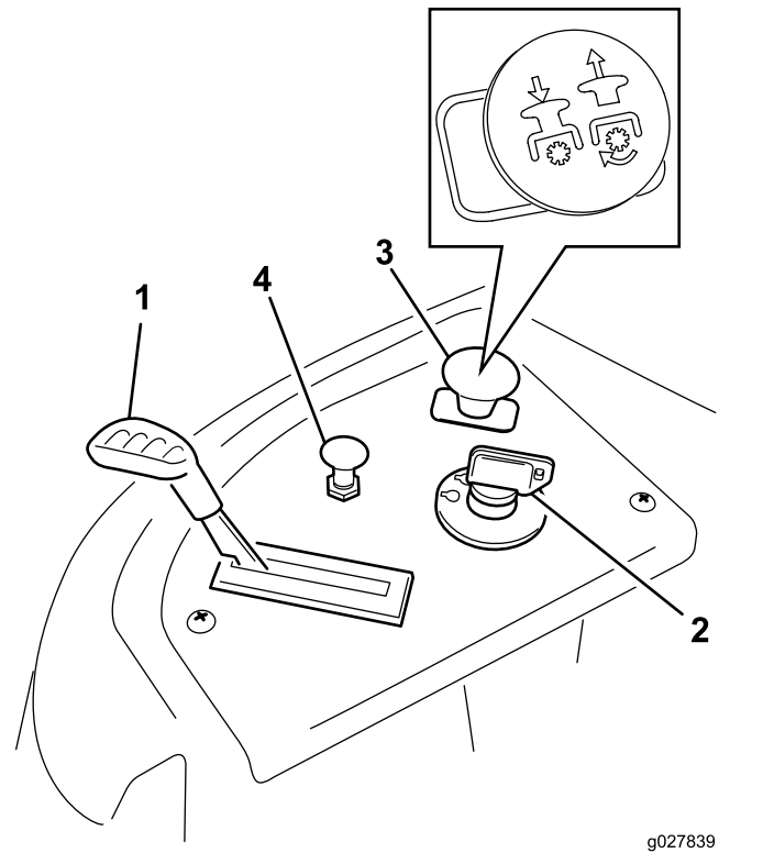
Figure 5 Control Panel
