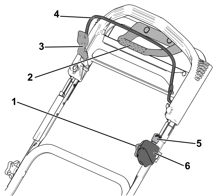
Figure 9 Upper handle
