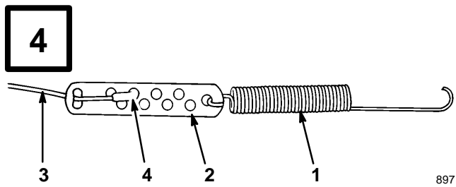
1. Spring 2. Cable adjuster 3. Cable 4. Z fitting
