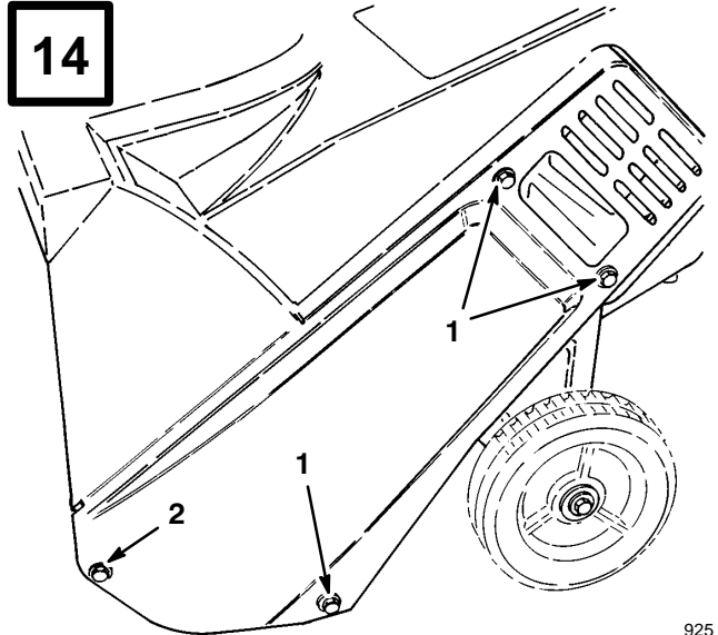
1. Self-tapping screws 2. Capscrew, nut, washer
