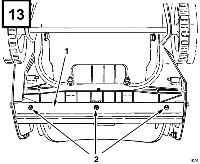
1. Scraper 2. Screws
