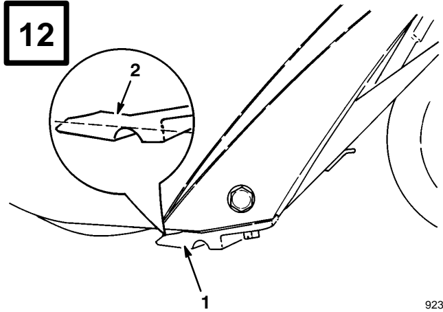
1. Scraper 2. Wear indicator groove
