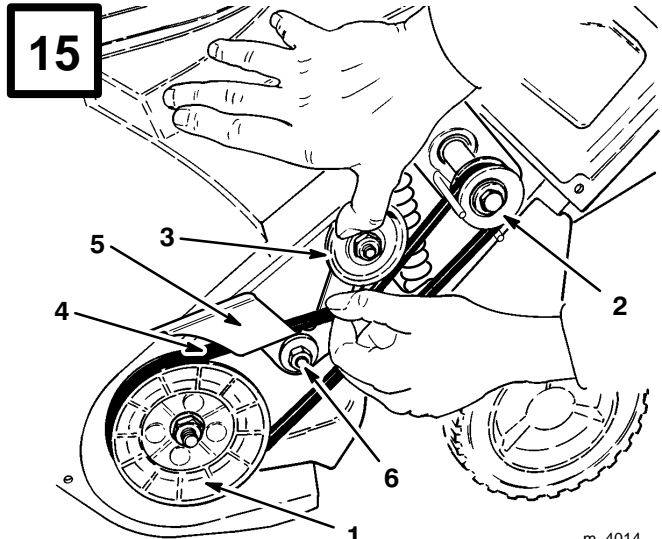
1. Rotor pulley 2. Drive pulley 3. Idler pulley 4. Drive belt 5. Brake arm 6. Idler pivot nut
