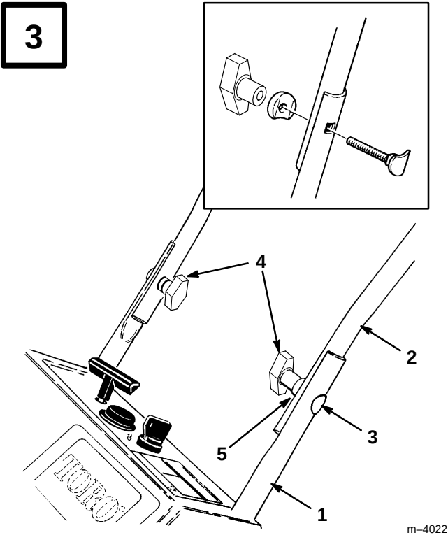
1. Lower handle 2. Upper handle 3. Oval head bolt 4. Knob 5. Curved washers
