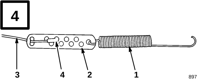
1. Spring 2. Cable adjuster 3. Cable 4. Z fitting
