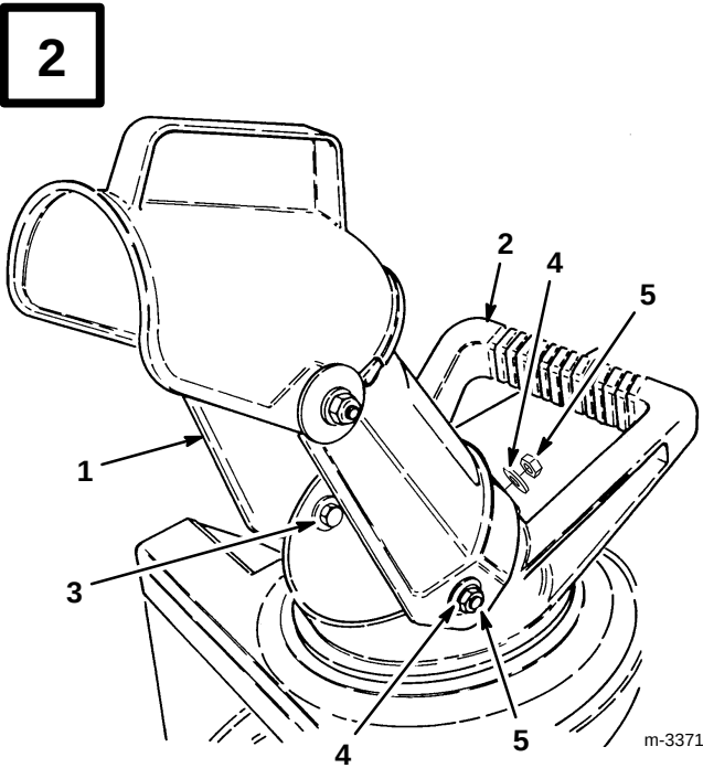
1. Discharge chute 2. Chute handle 3. Hex bolt 4. Washer 5. Locknut
