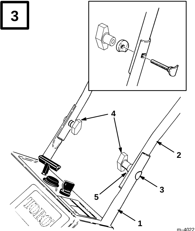
1. Lower handle 2. Upper handle 3. Oval head bolt 4. Knob 5. Curved washers
