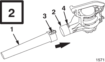
1. Blower tube 2. Blower housing outlet 3. Tab 4. Latch
