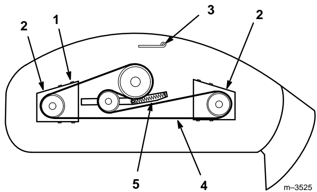
Figure 36 Top View
