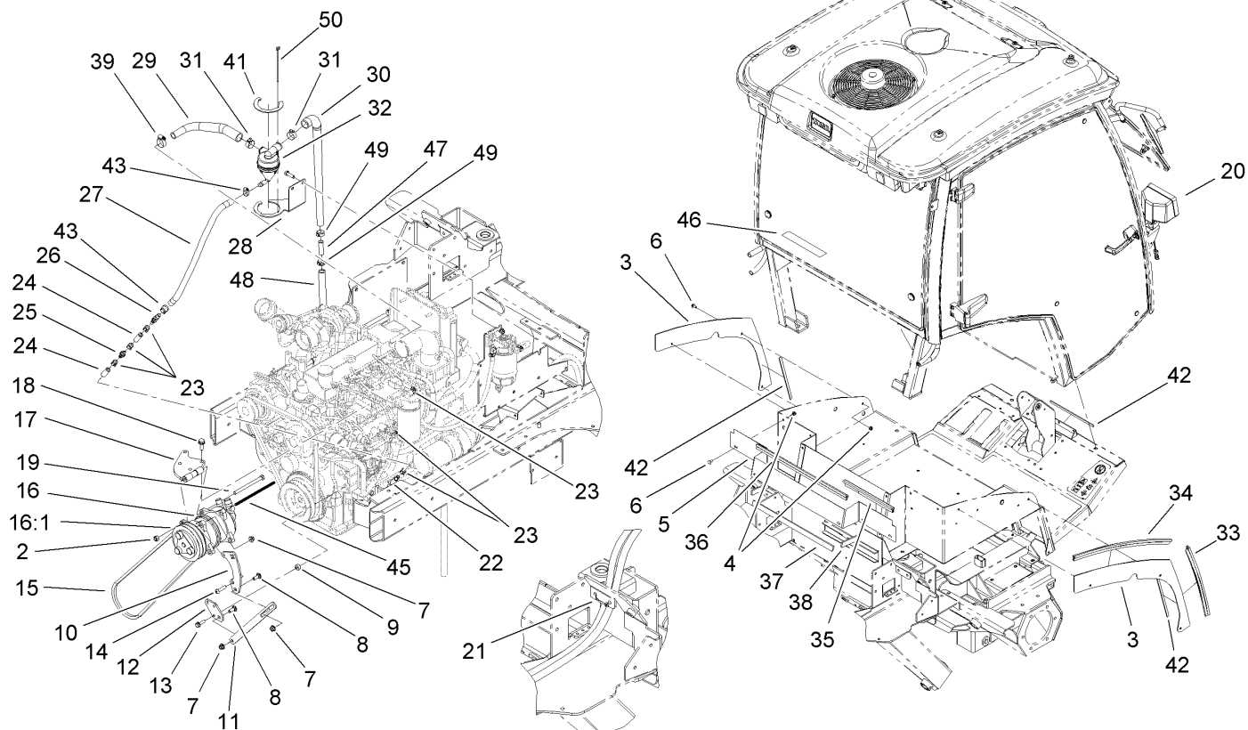
VIEW OF A/C HOSE ROUTING
