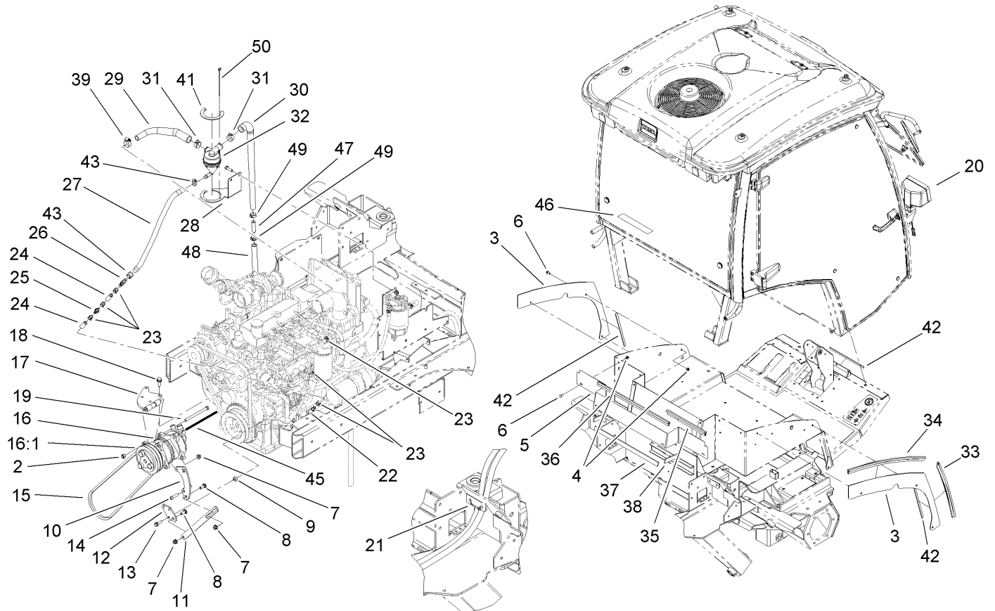
VIEW OF A/C HOSE ROUTING
