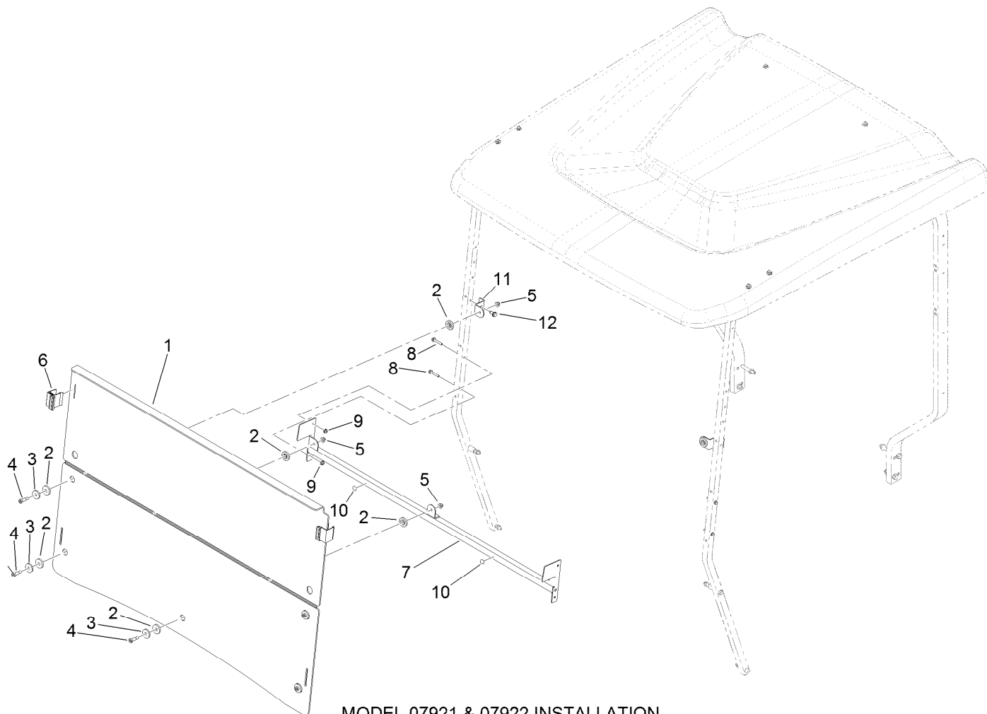
MODEL 07921 & 07922 INSTALLATION
