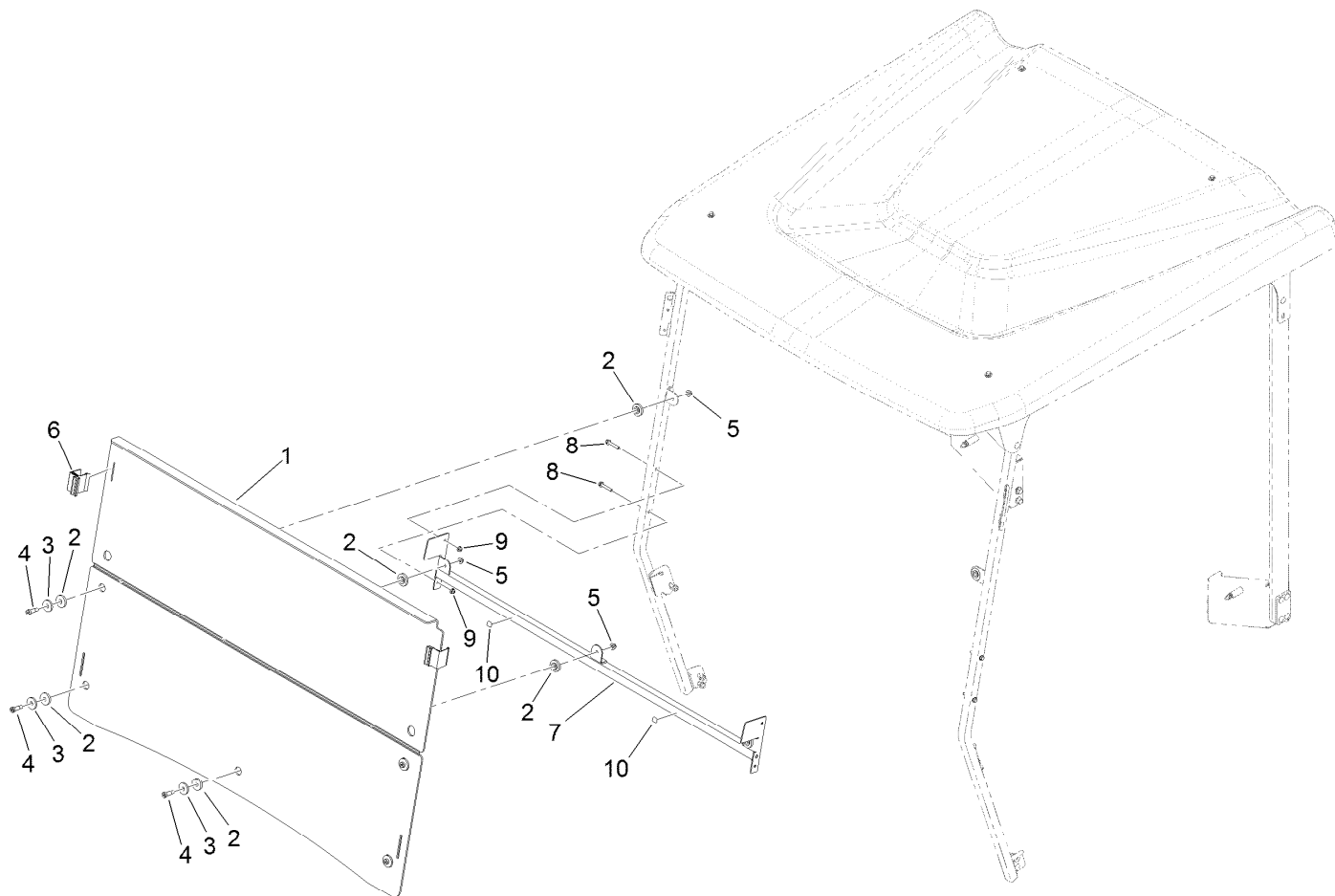
MODEL 07140 & 07141 INSTALLATION
