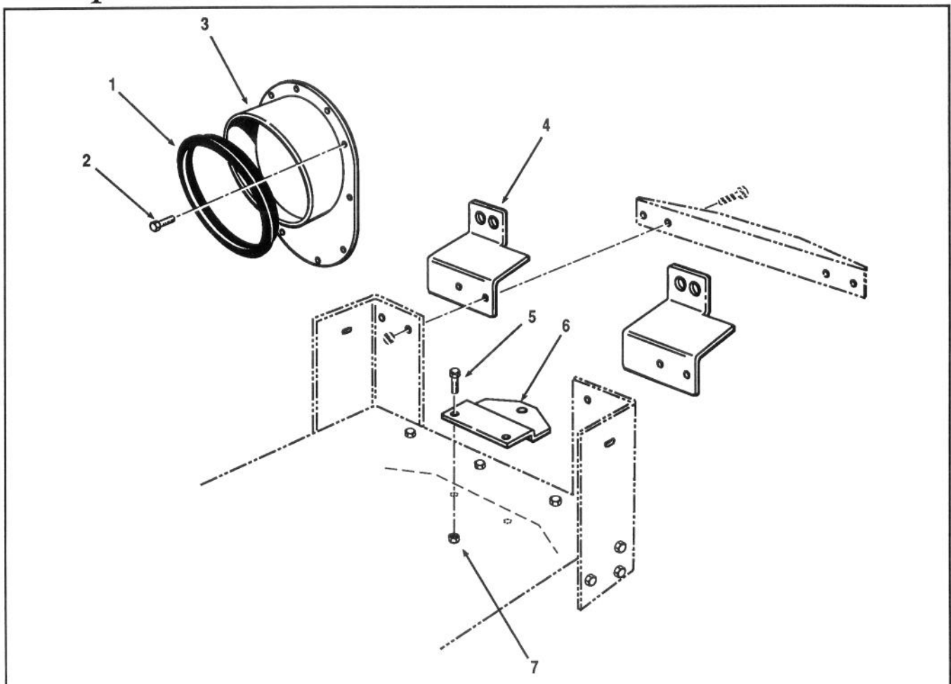
EASY EMPTY ADAPTER KIT PART NUMBER 80-2190
