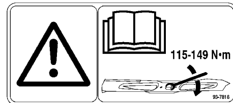
ON TOP OF CUTTING UNIT (Part No. 93-7818)
