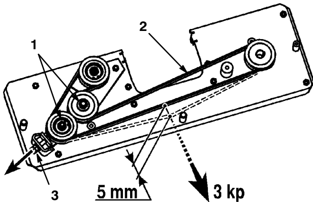
Figure 42 Top View
