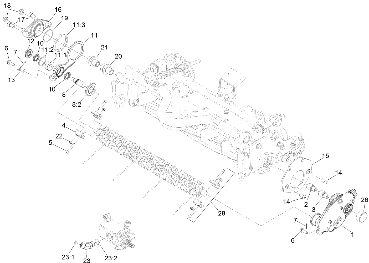
RM3550/55 Front Center Cutting Unit Only
