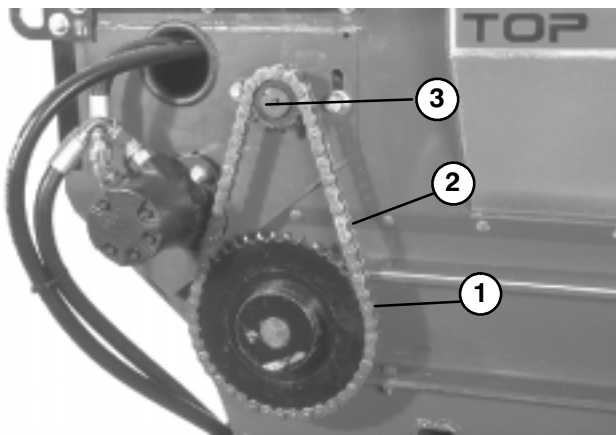
Figure 23 1. Drive chain 2. Master link 3. Motor
