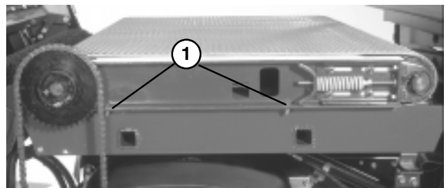
Figure 27 1. Slider bed mounting capscrews
