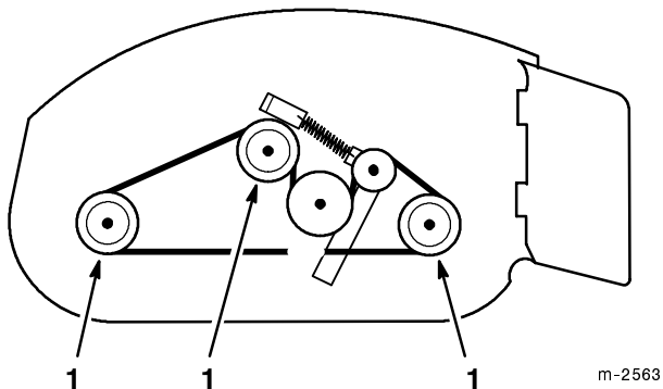
Figure 21 Top View
