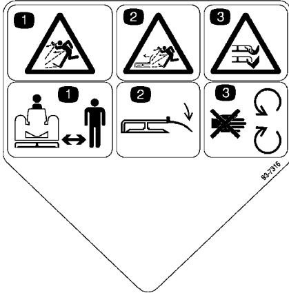
Part No. 93-7316
