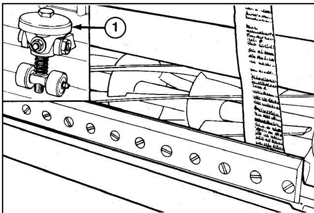
Figure 1 1. Bedknife adjusting knob
