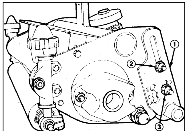
Figure 2 1. Rear height of cut bracket 2. Top capscrew and nut 3. Bottom nut
