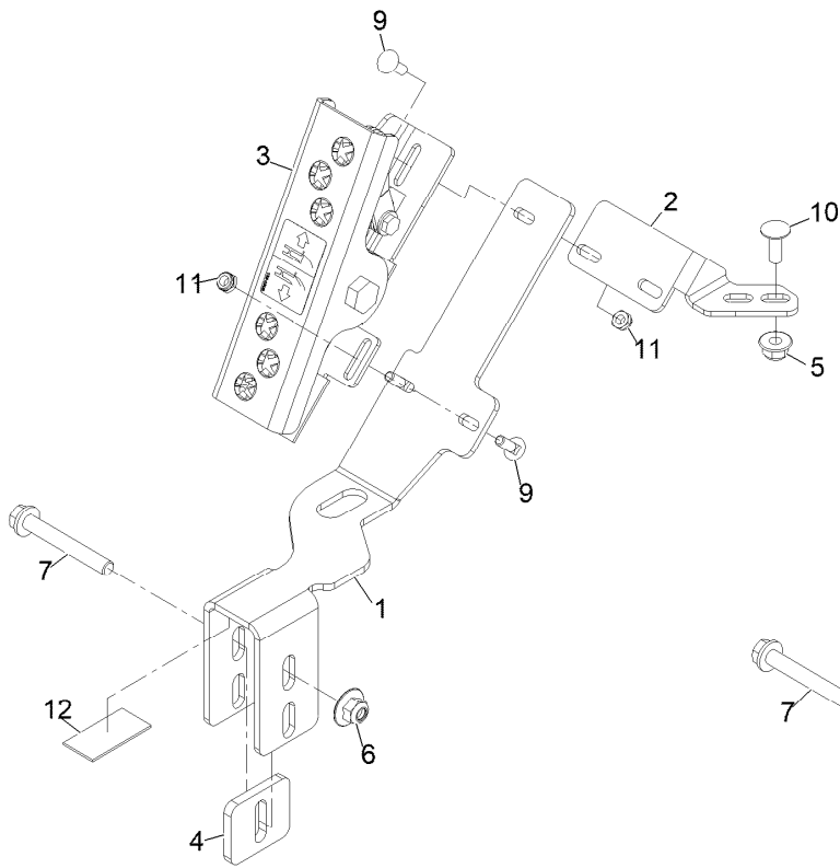
LAZER WITH FULL SUSPENSION PLATFORM
