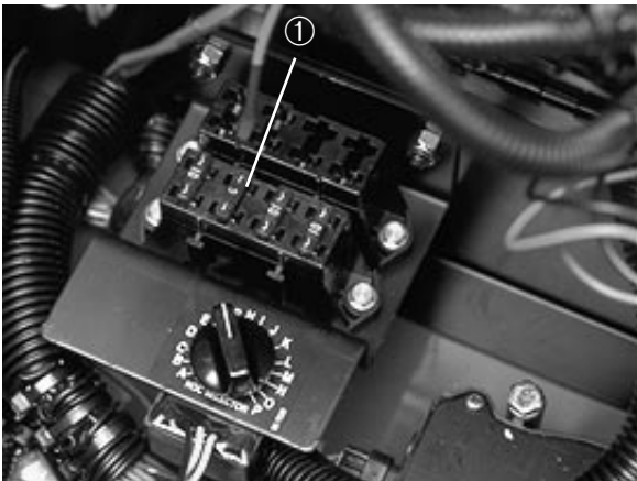
Figure 56 1. Fusibles
