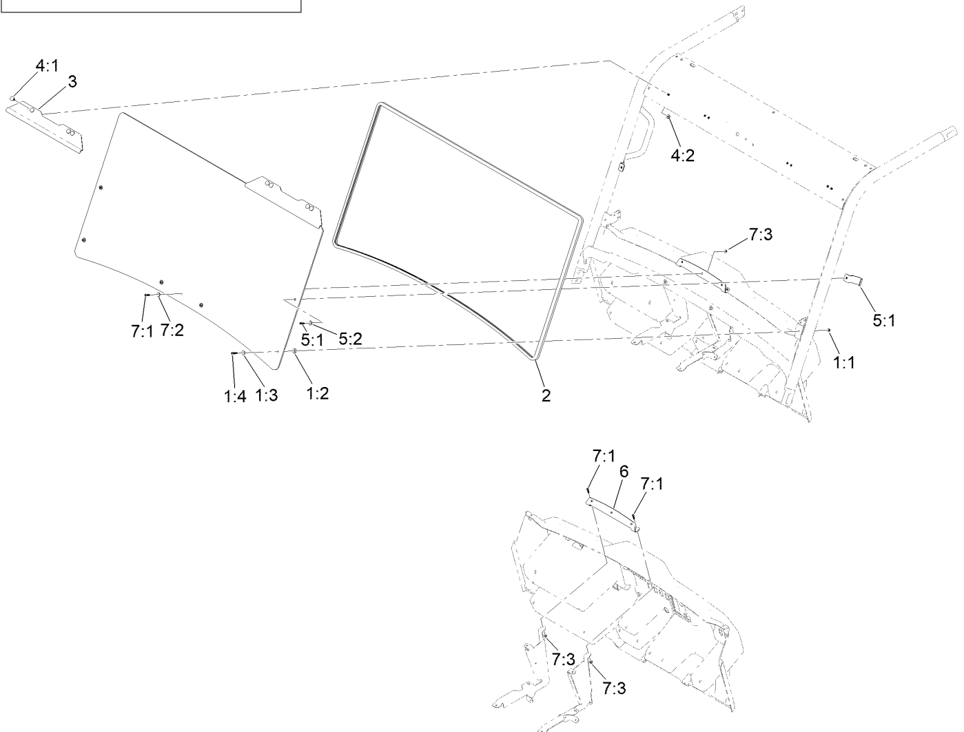
LOWER WINDSHIELD BRACKET INSTALLATION
