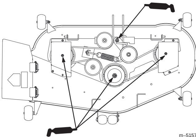
Figure 30 Top View
