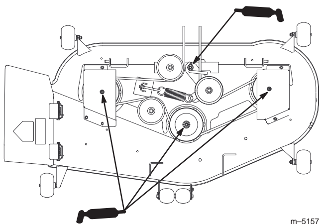
Figure 30 Top View
