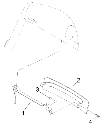
MODEL 07142 CAB
