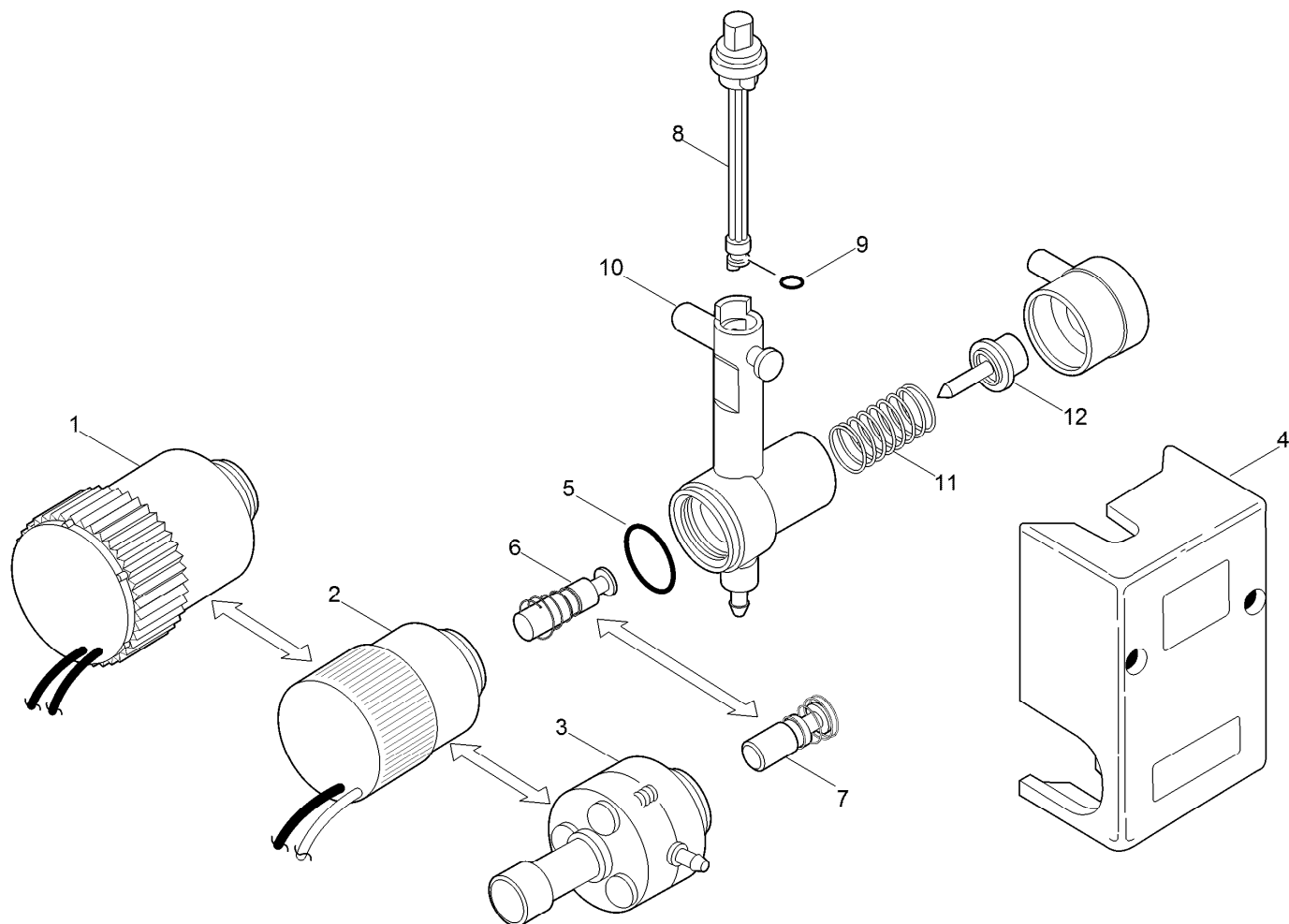
Pilot Valve, Fixed Pressure - 600 and 700 Series (continued)
