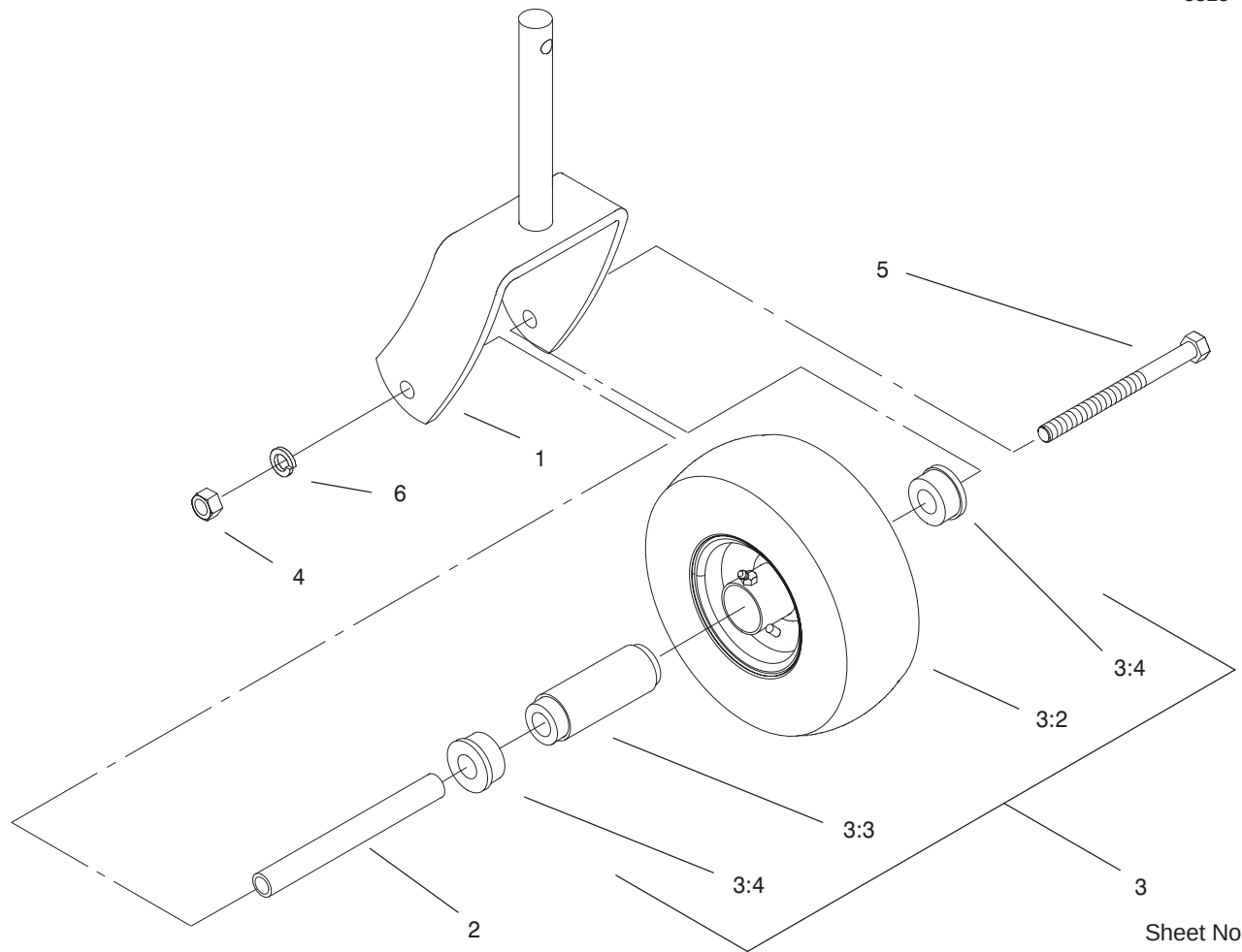
Caster and Wheel Assembly No. 1-322154
