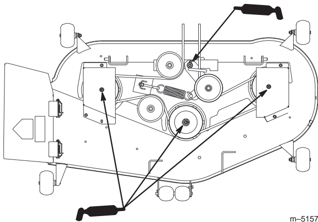
Figure 31 Top View
