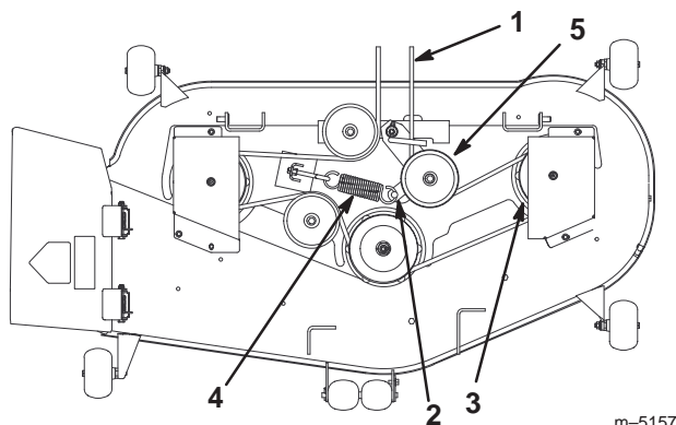
Figure 44 Top View
