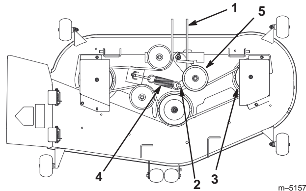
Figure 44 Top View
