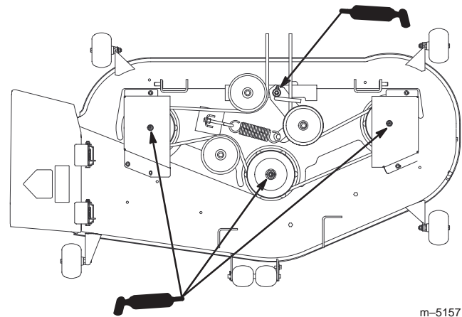
Figure 30 Top View
