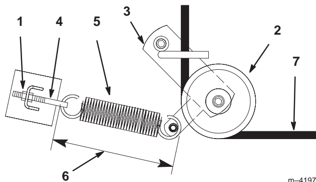
Figure 43 Top View
