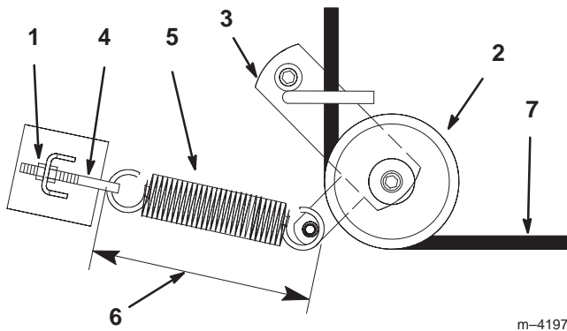
Figure 43 Top View
