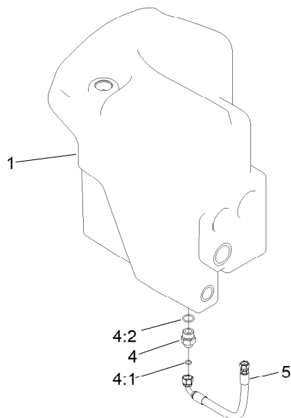
RM50XX AND GM4300 HYDRAULIC MODEL COMPONENTS
