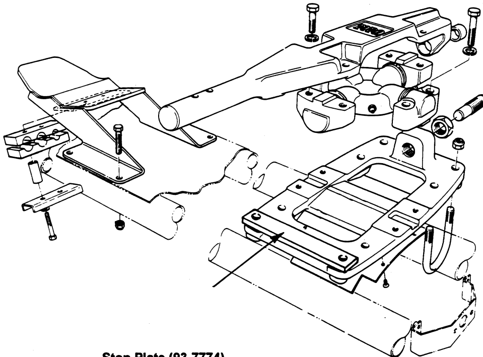
Note: Controls forward motion to prevent Cutting Unit and Lift Cylinder contact.
