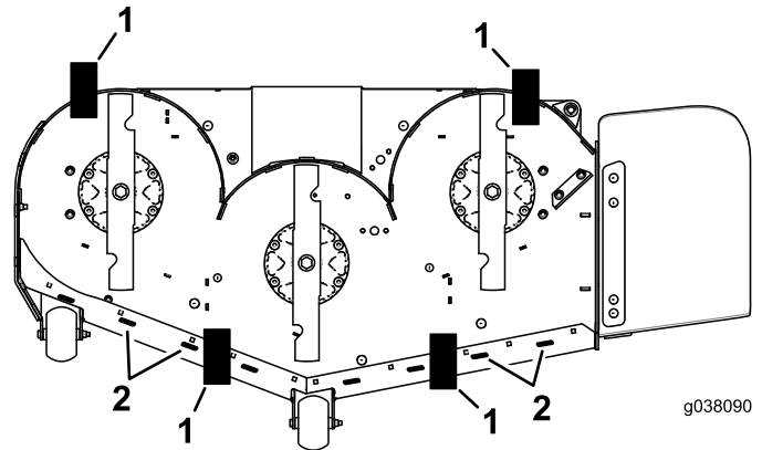
Figure 90 Bottom view
