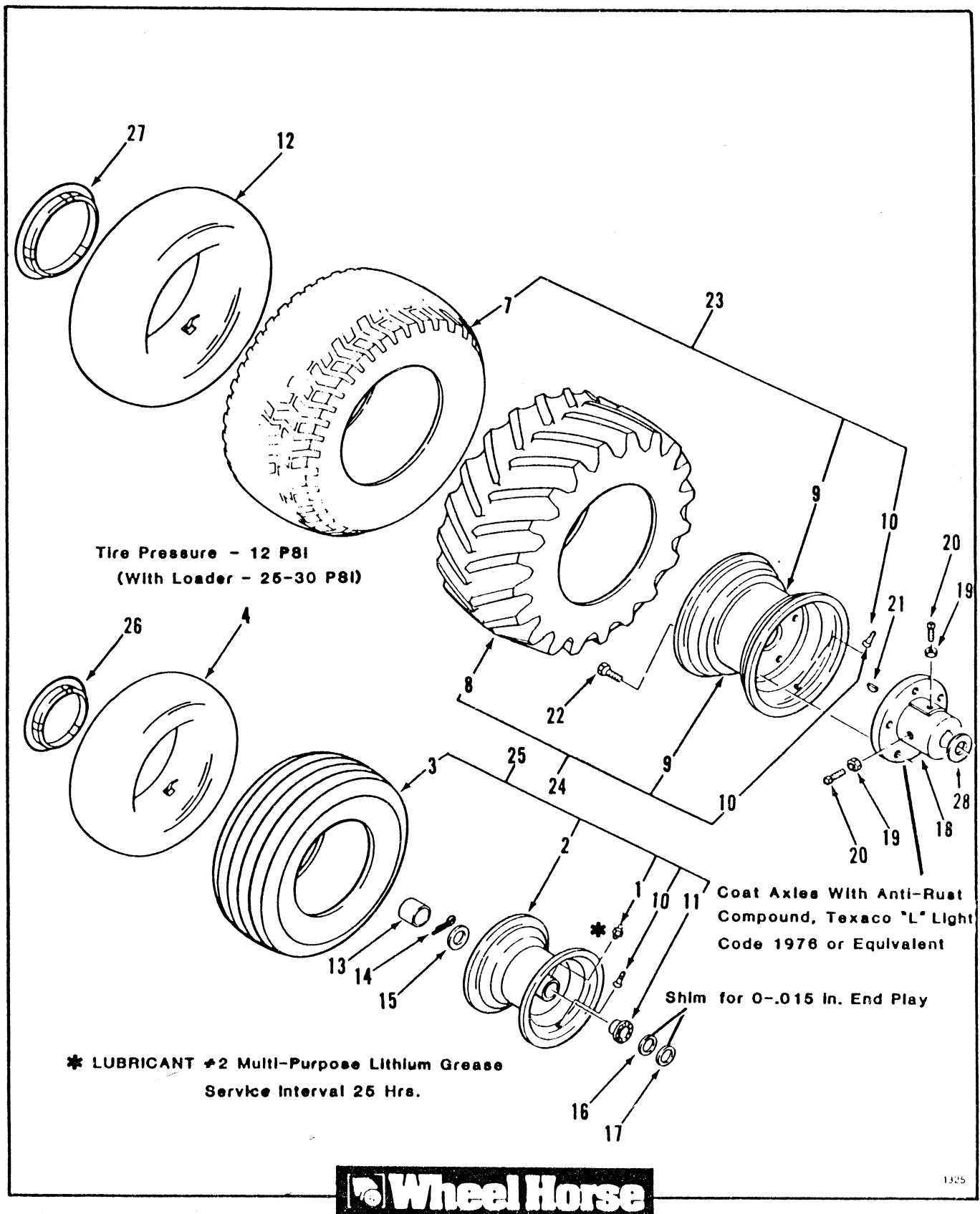
Figure 13-1 Wheels and Tires
