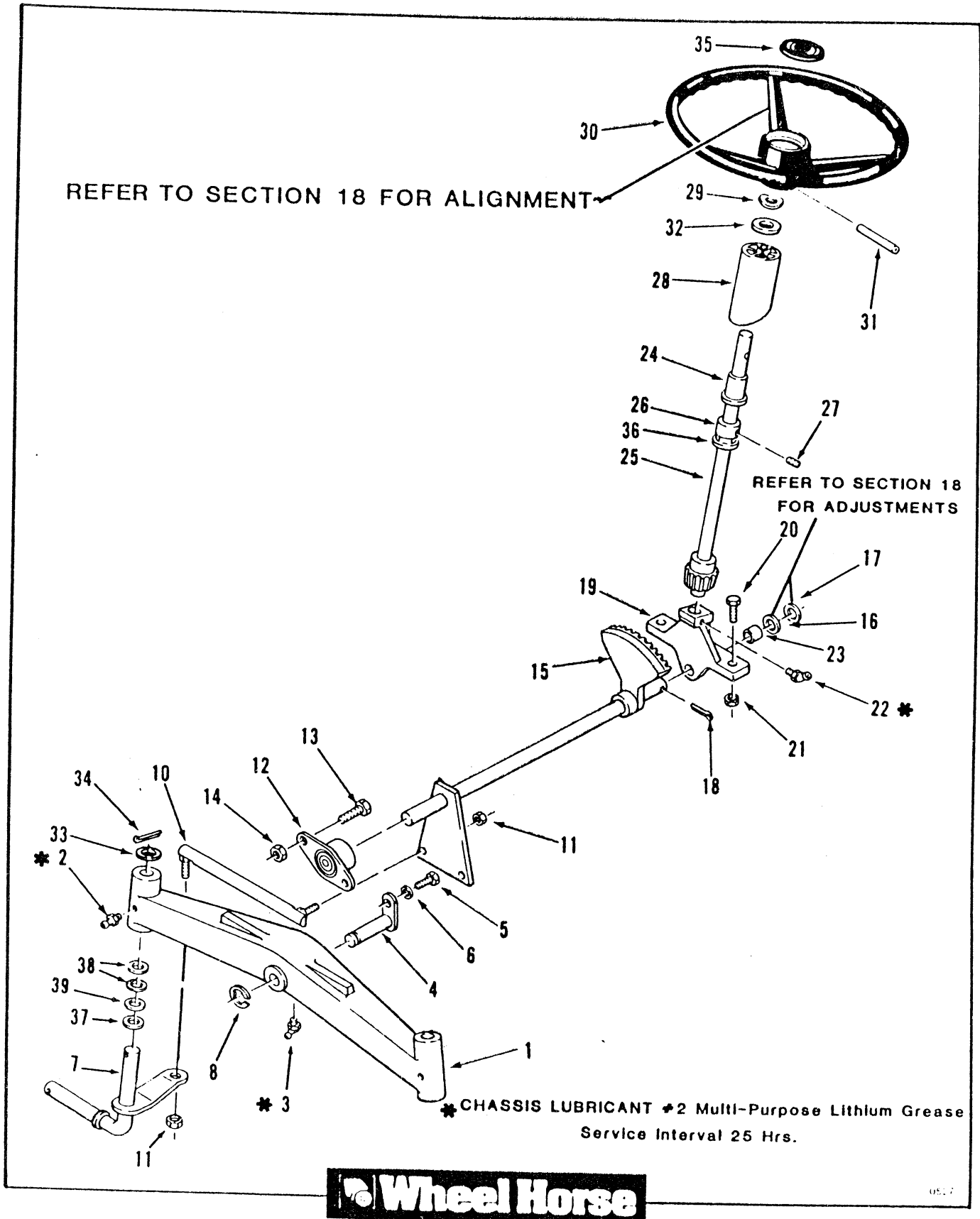
Figure 5-1 Front Axle and Steering
