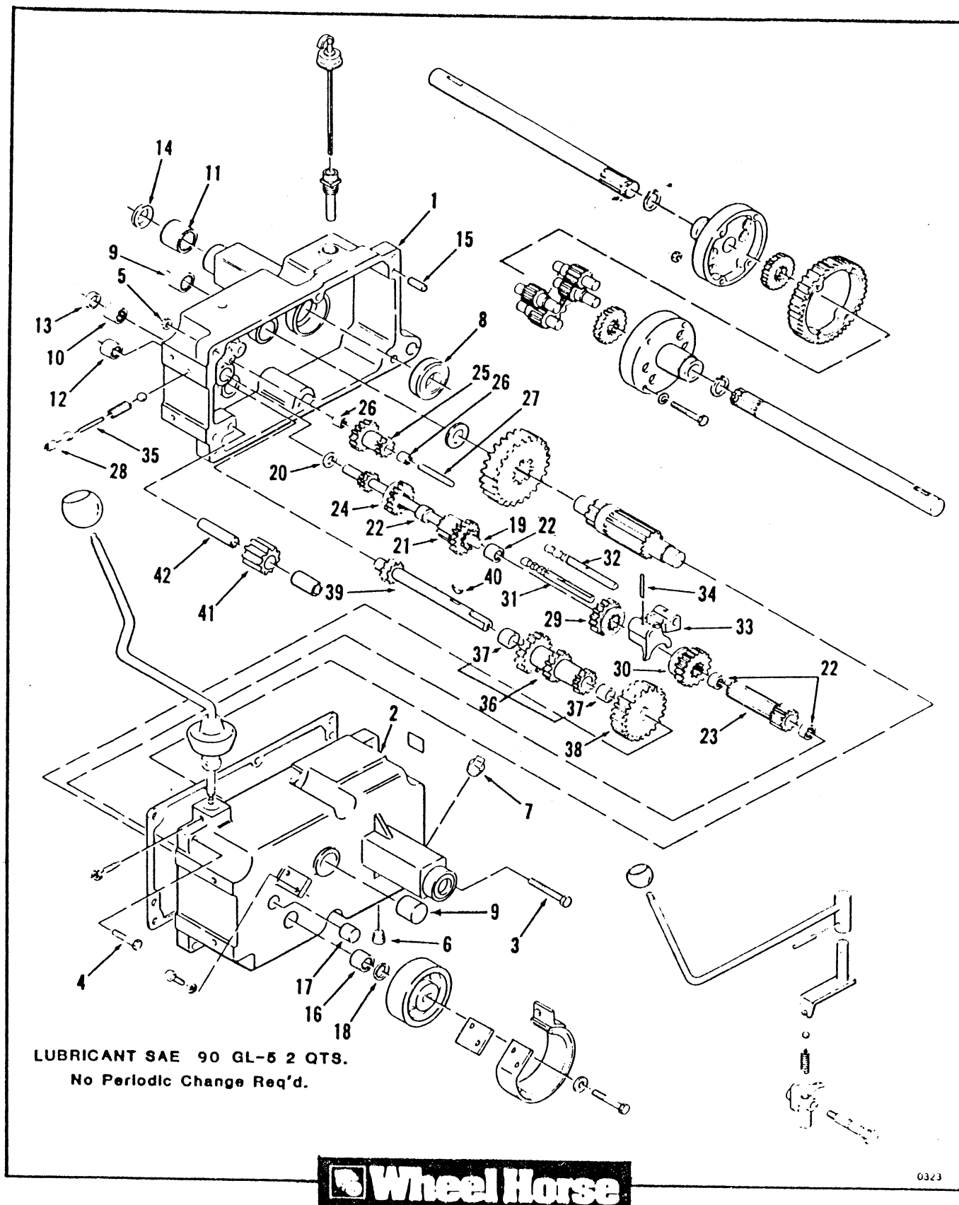
Figure 3-1 Mechanical Transmission - 8-Speed
