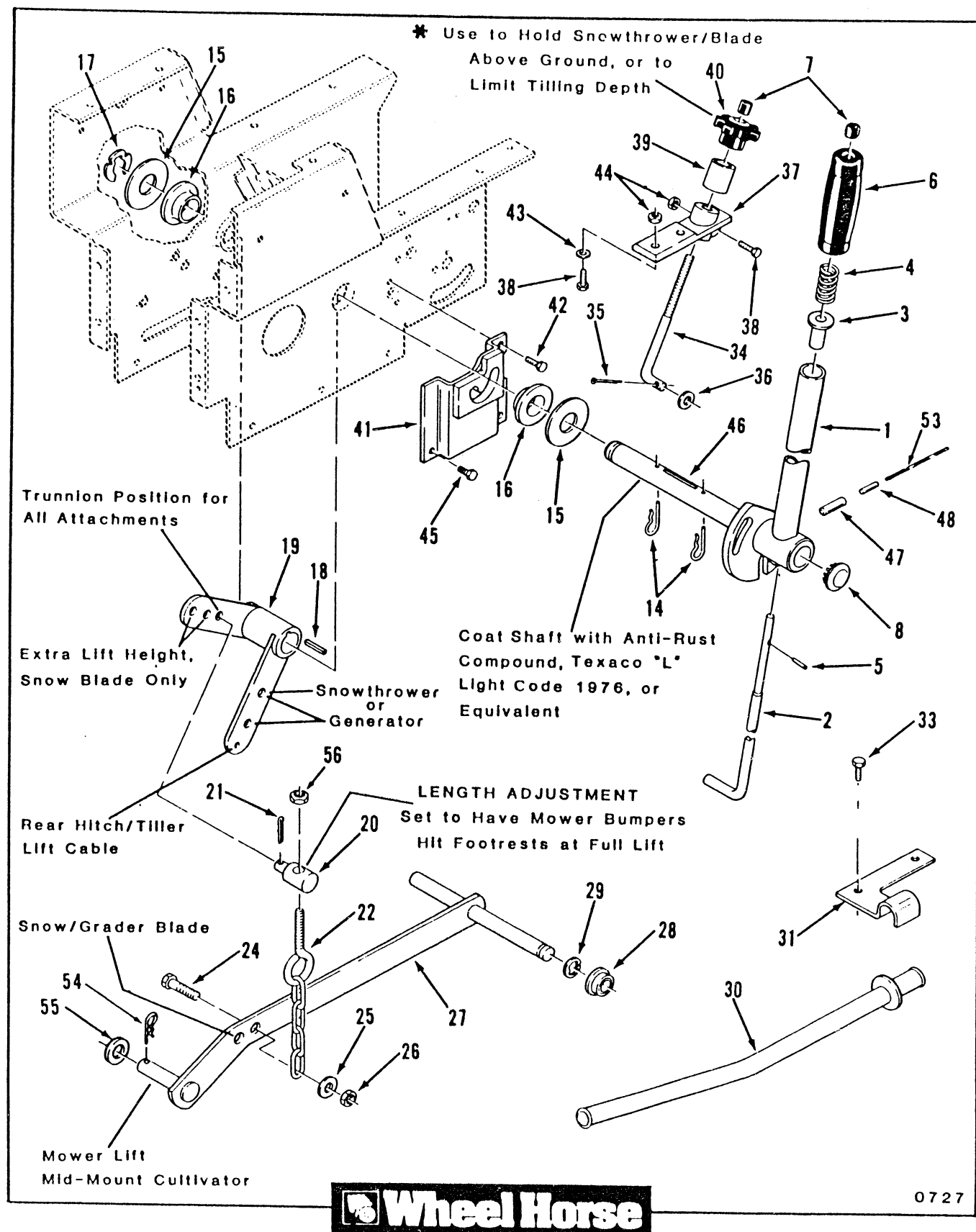
Figure 7-2 Lift Linkage
