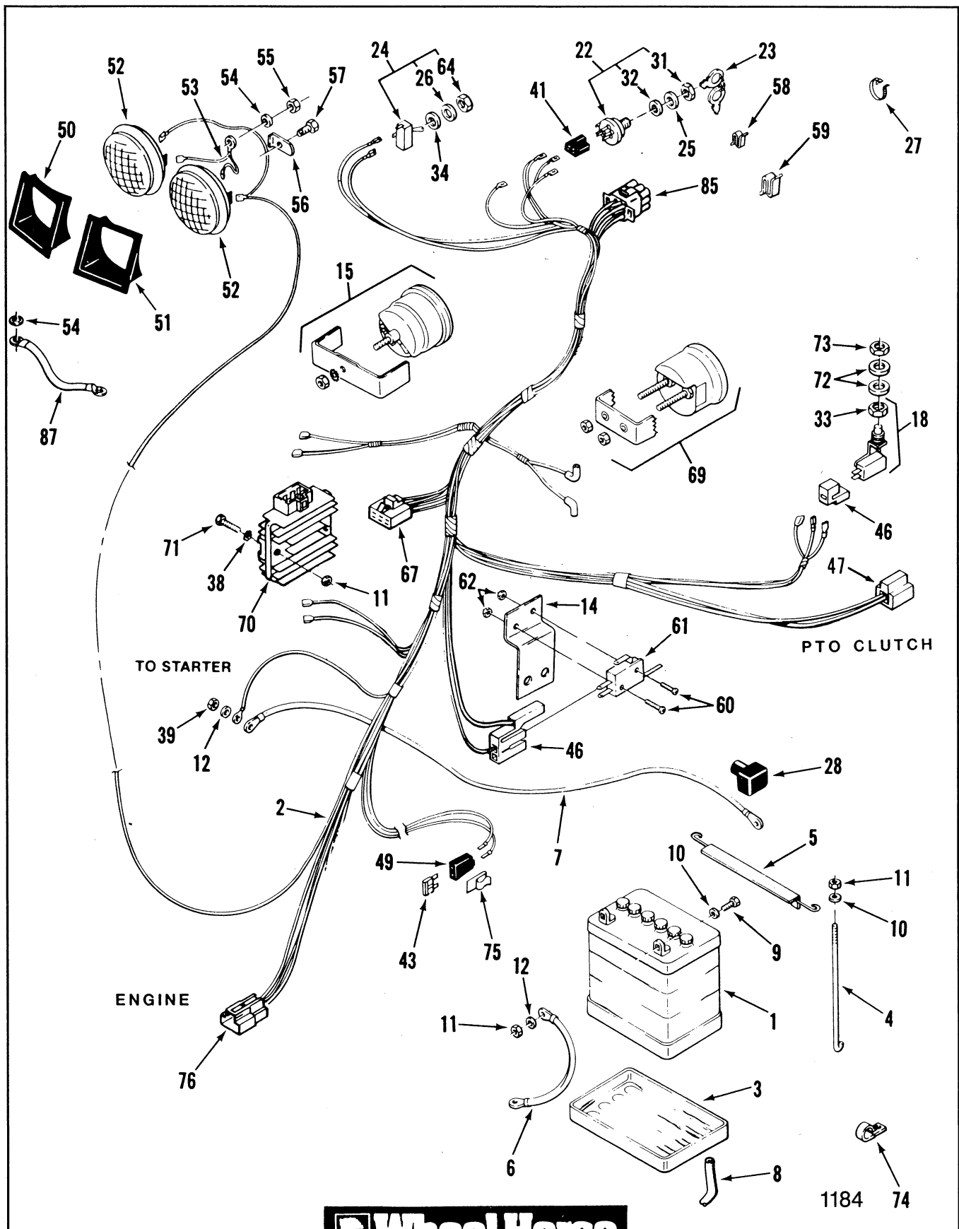
Figure 11-1 Electrical System
