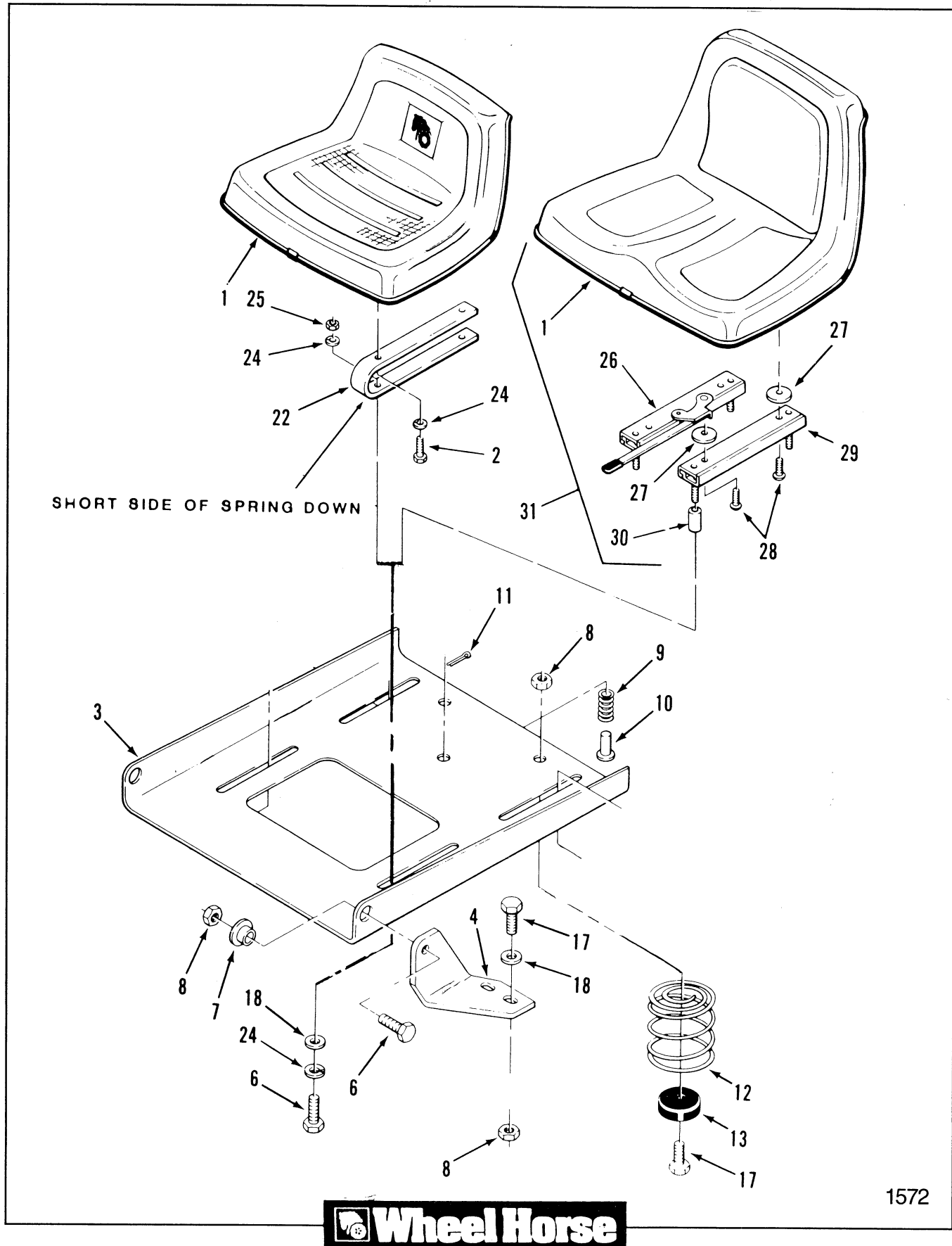
Figure 15-1 Seat and Suspension
