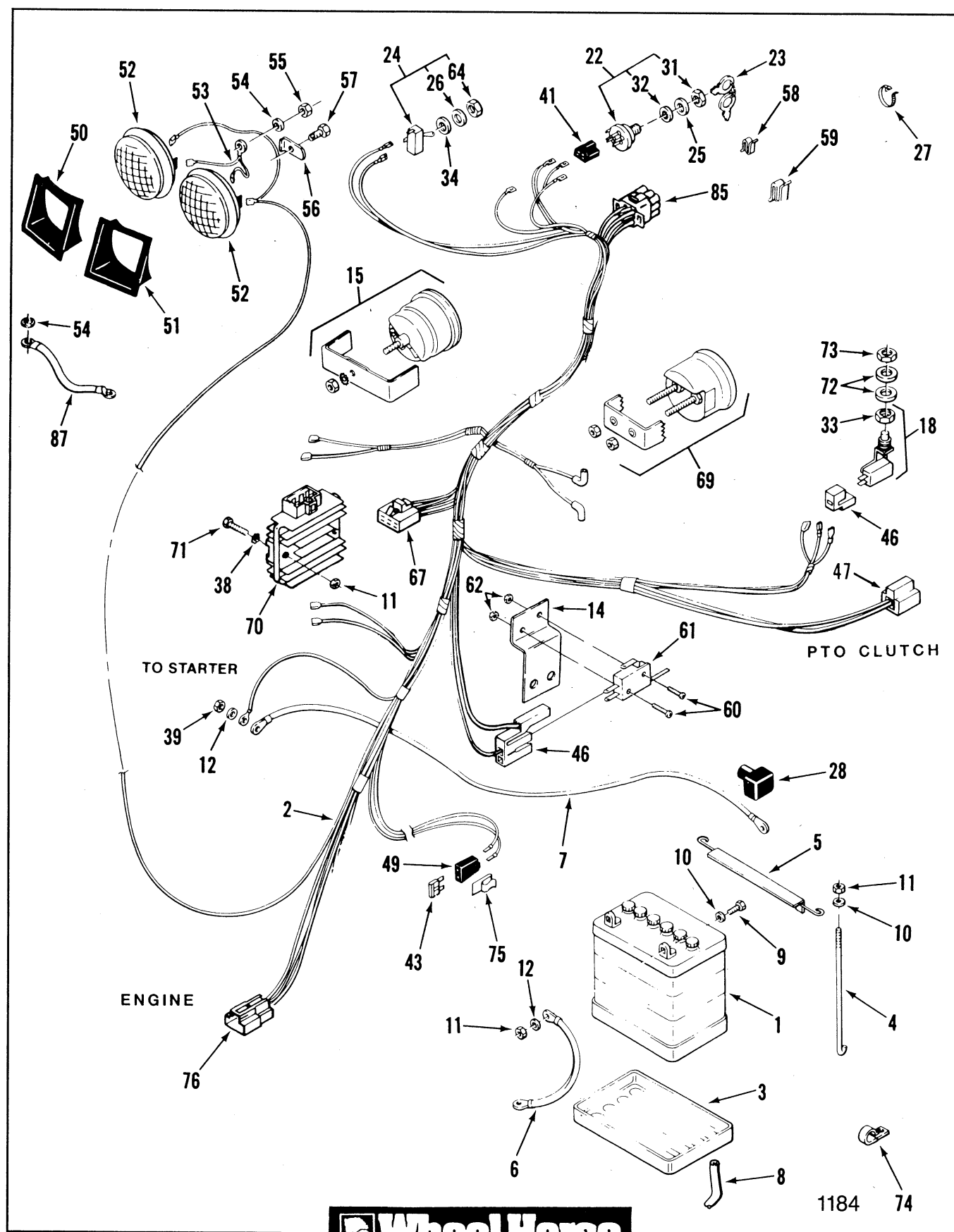
Figure 11-1 Electrical System
