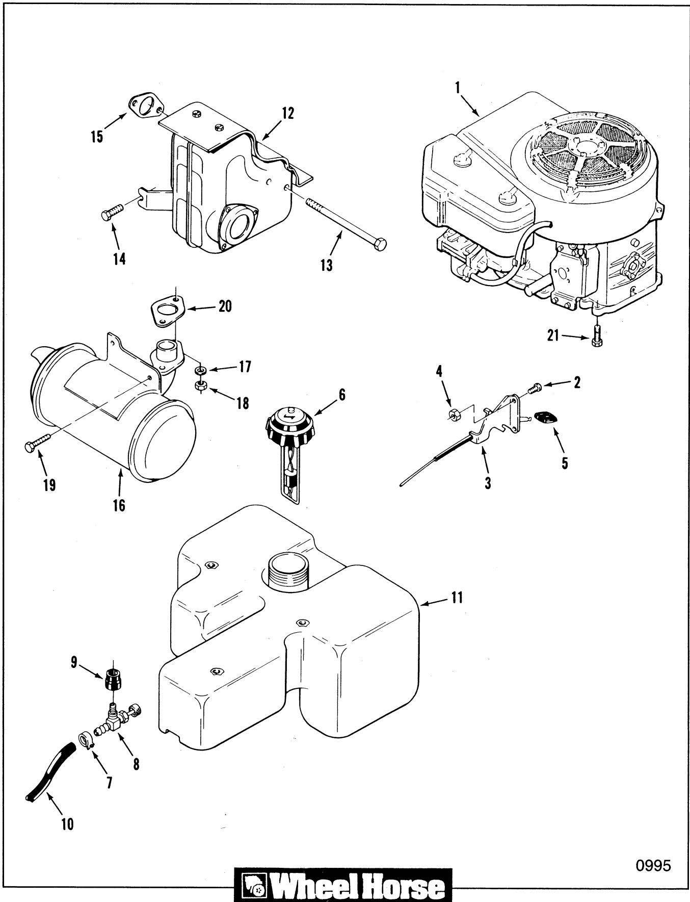
Figure 9-1 Engine, Fuel &amp; Exhaust Systems
