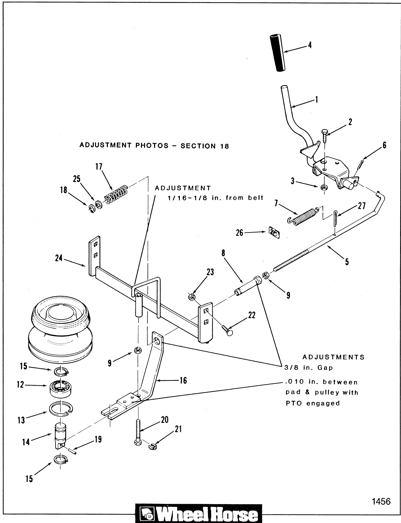
Figure 14-2 PTO Clutch
