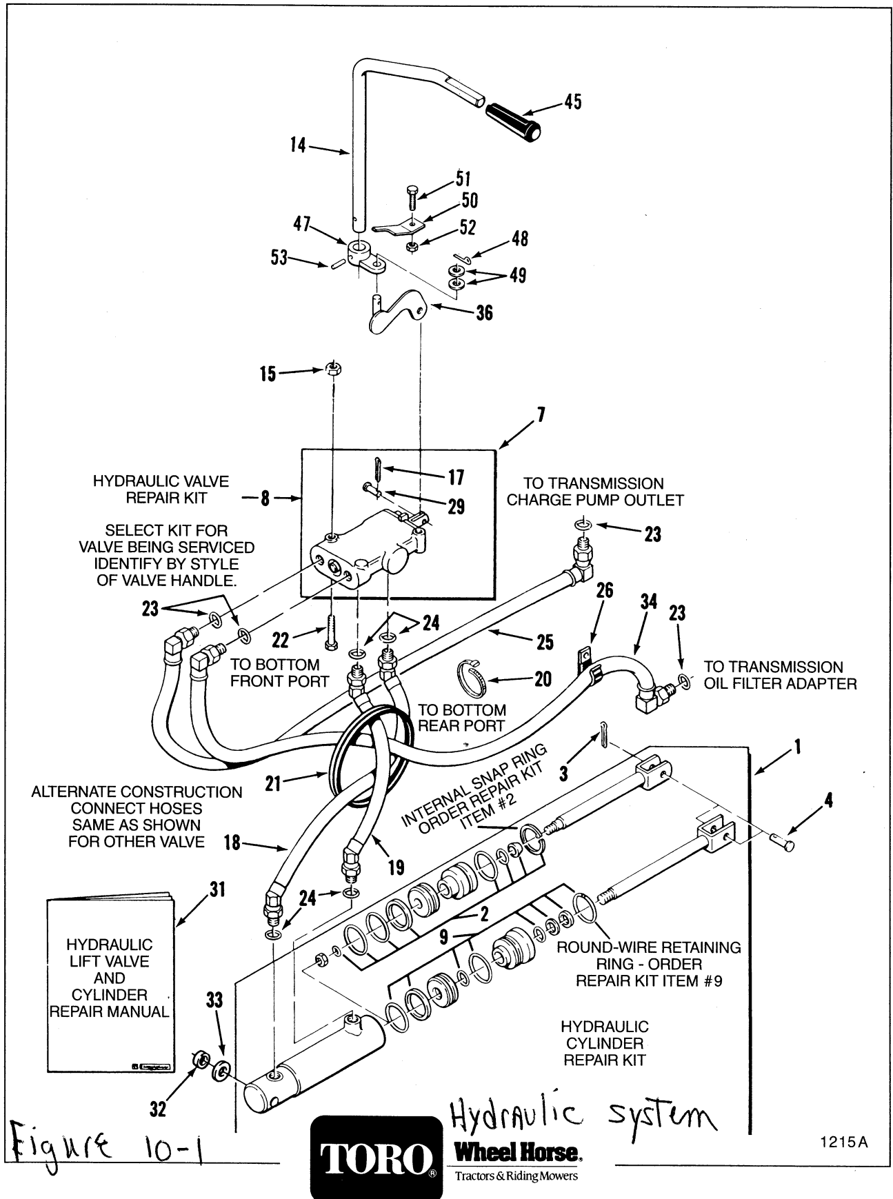
Figure 10-1 Hydraulic System
