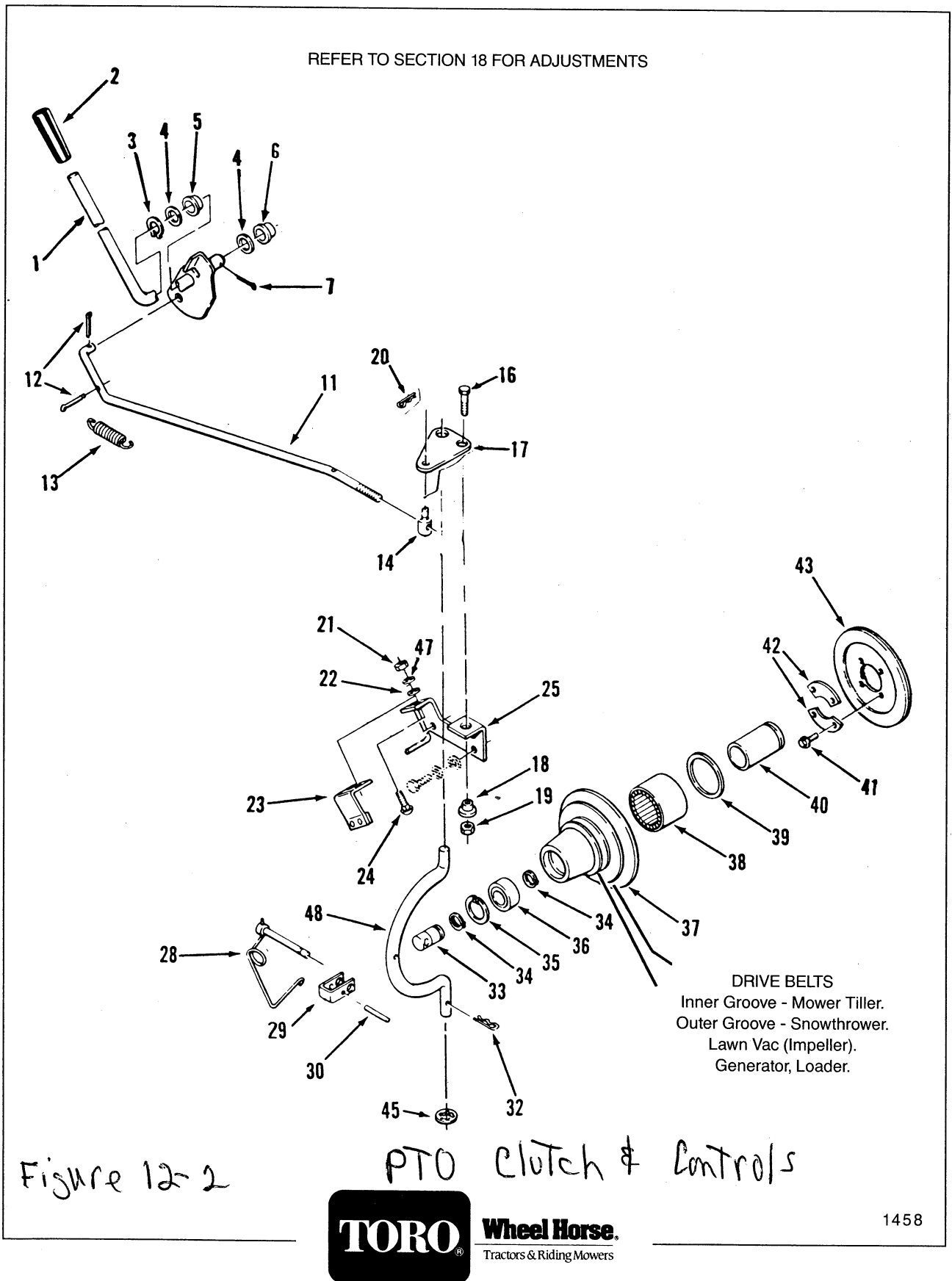
Figure 12-2 PTO Clutch and Control
