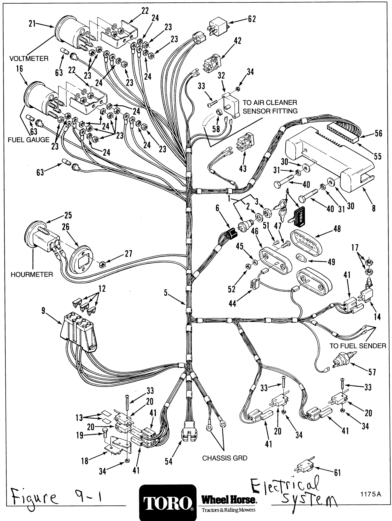
Figure 9-1 Electrical System
