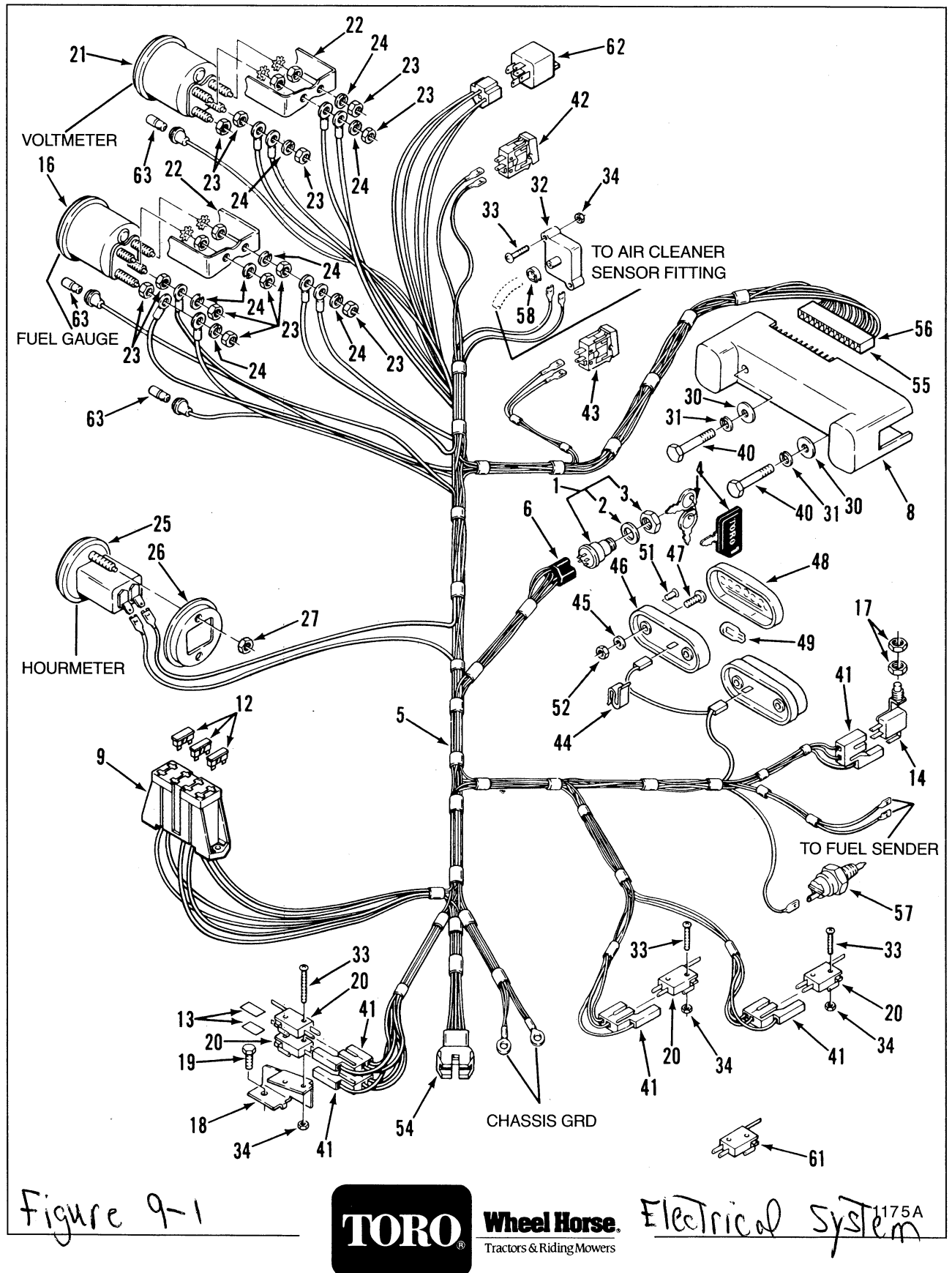
Figure 9-1 Electrical System
