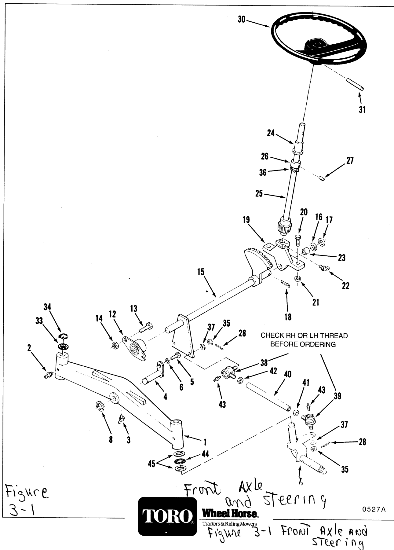
Figure 3-1 Front Axle and Steering
