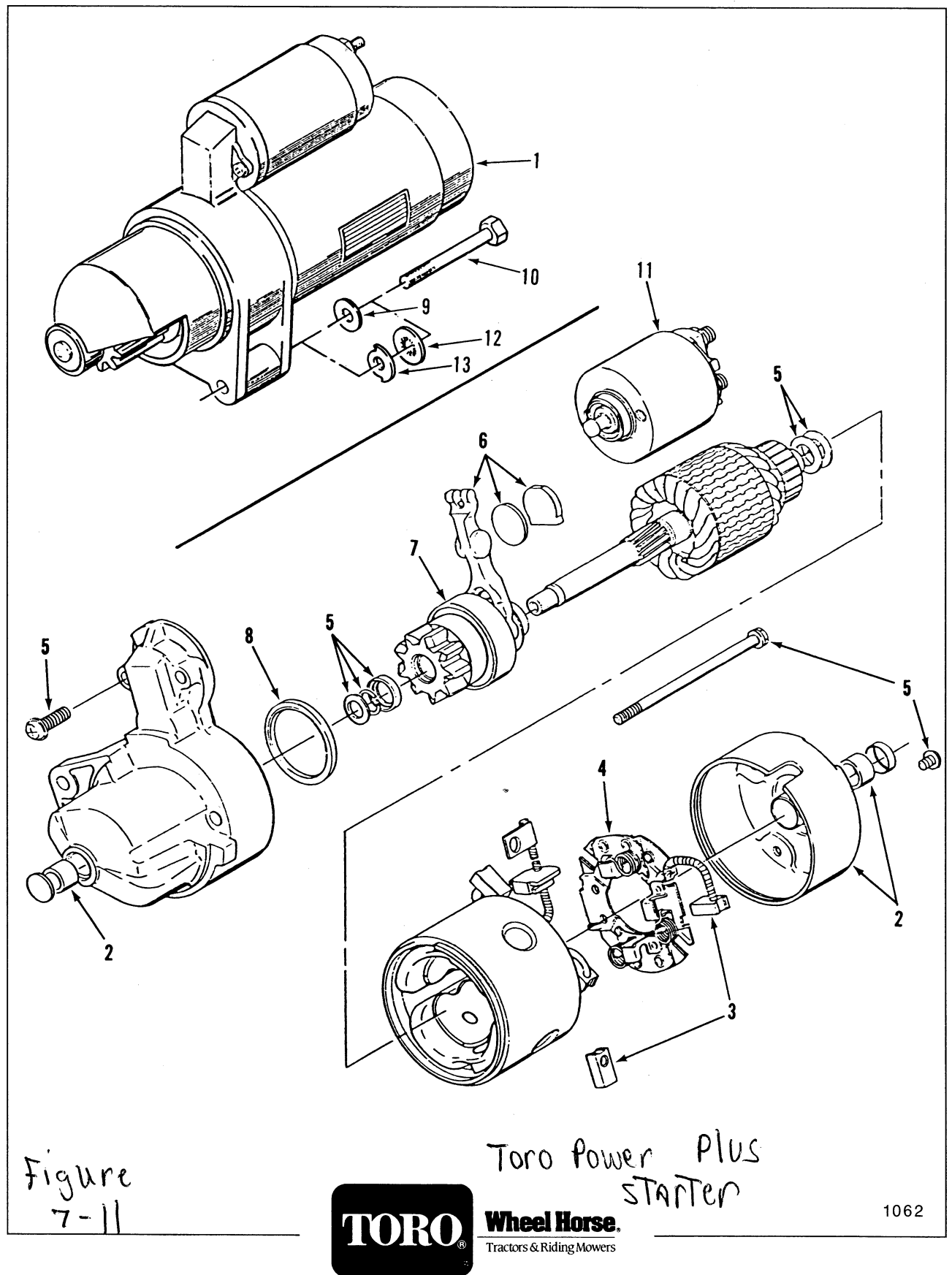
Figure 7-11 Toro Power Plus Starter
