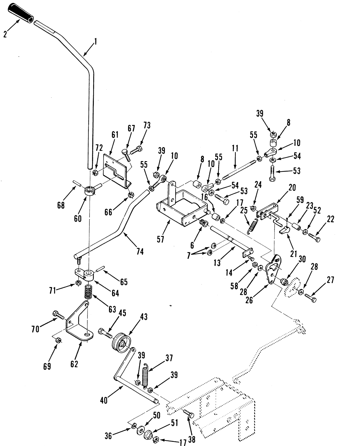
Figure 4-1 Clutch, Brake AND Figure 4-1
