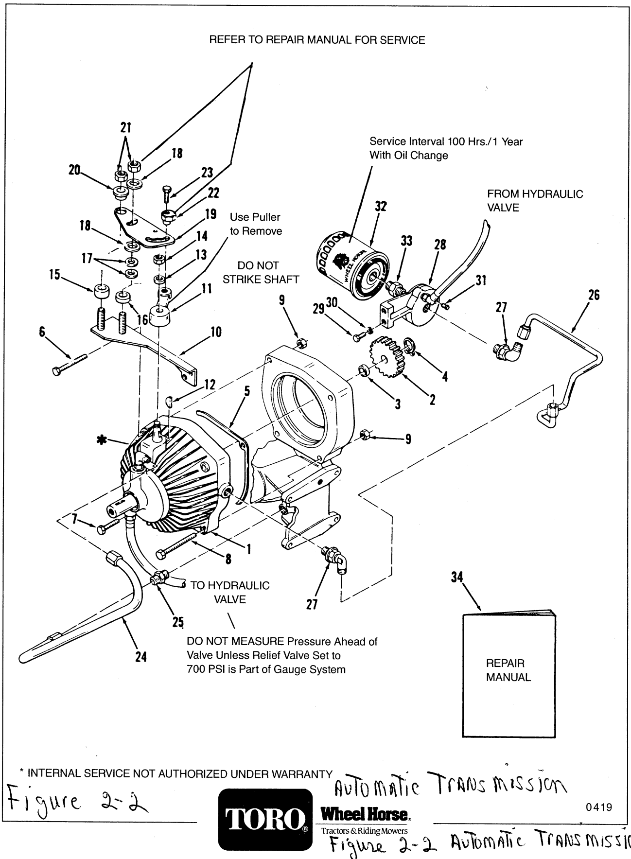
Figure 2-2 Automatic Transmission
