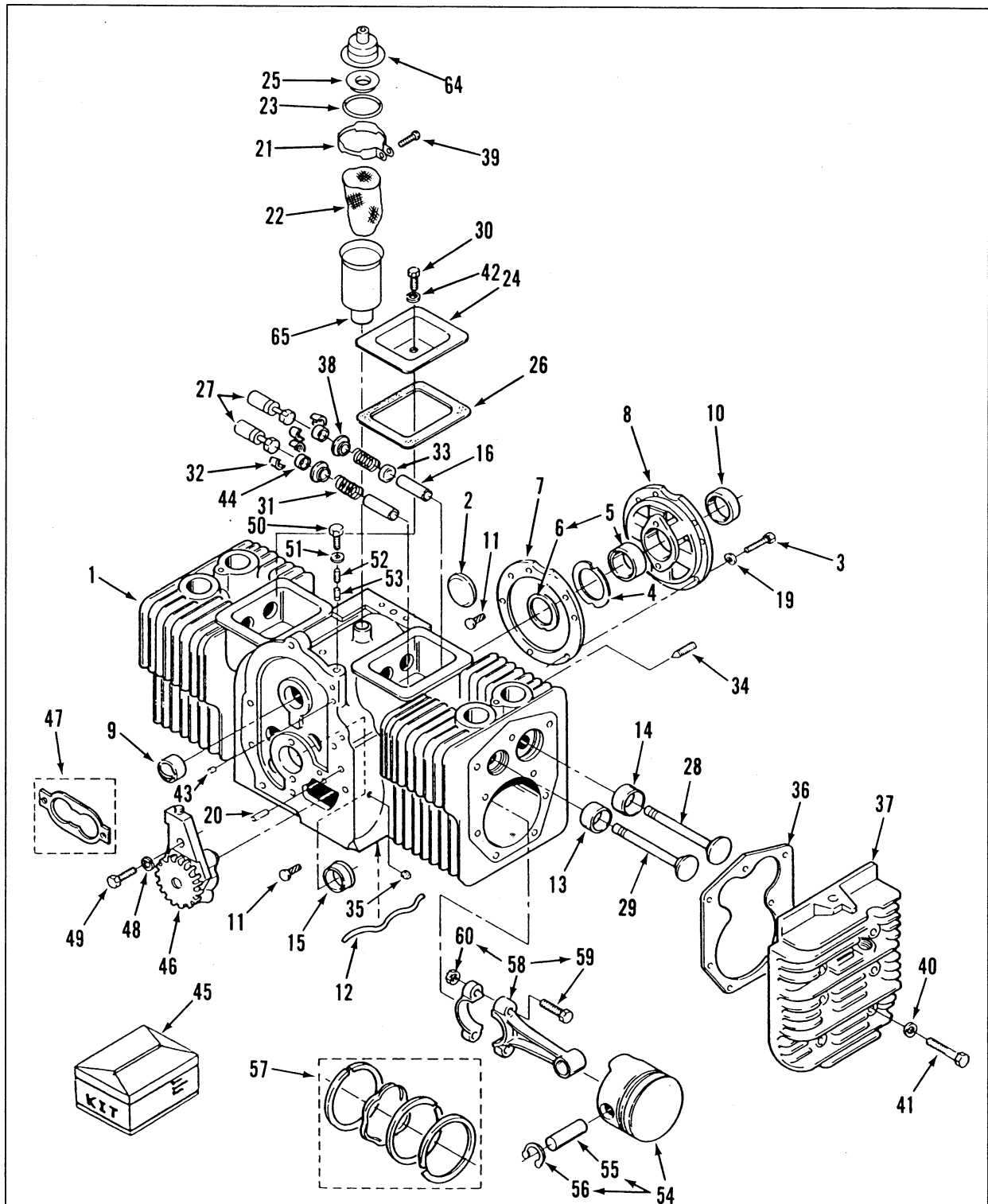
Figure 7-2 Toro Power Plus Figure 7-2 Toro
