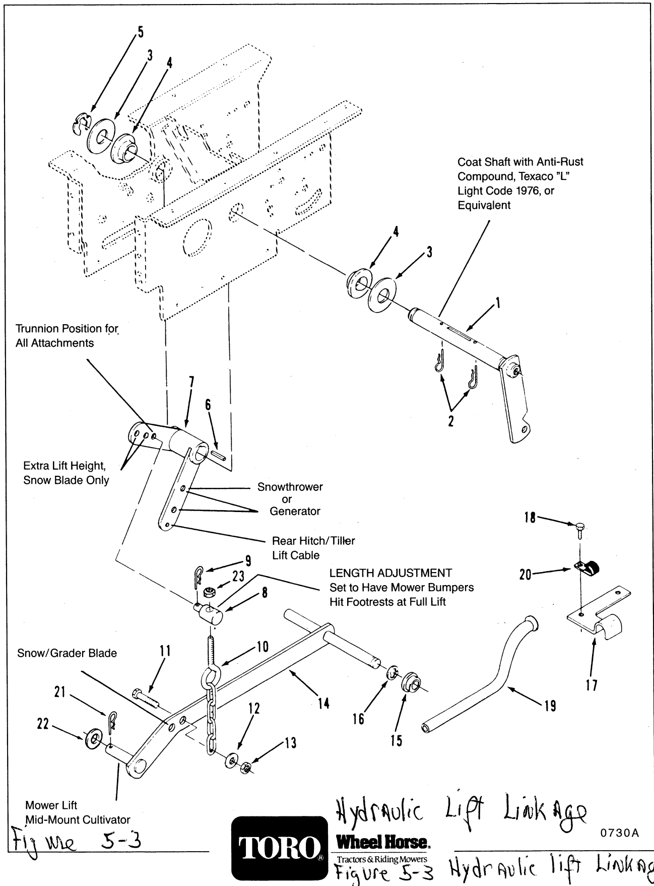
Figure 5-3 Hydraulic Lift Linkage
