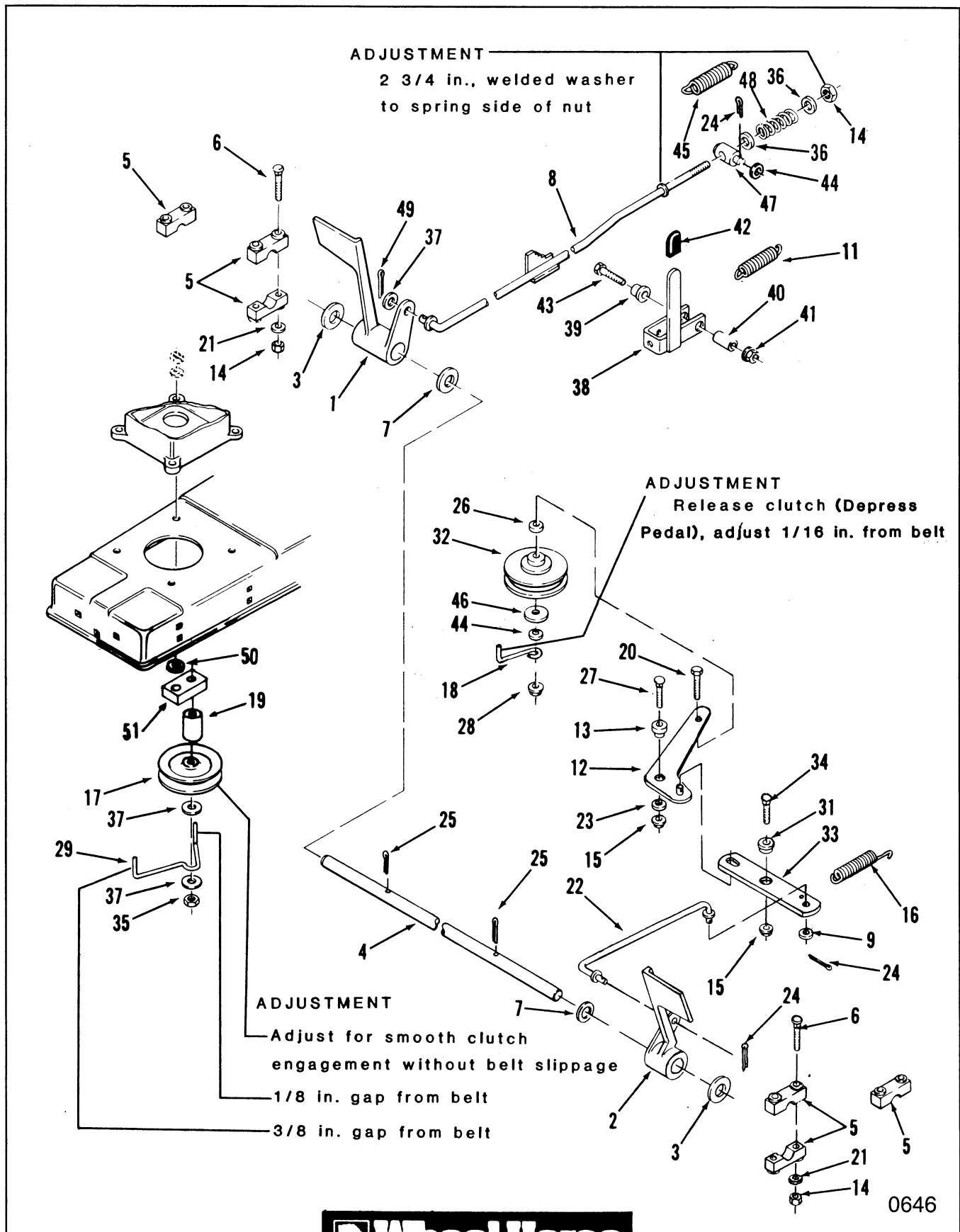
Figure 3-1 Brake and Clutch Linkage
