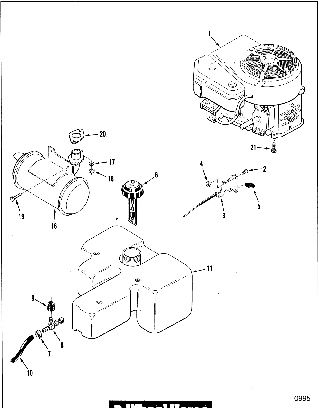
Figure 6-1 Engine, Fuel &amp; Exhaust Systems
