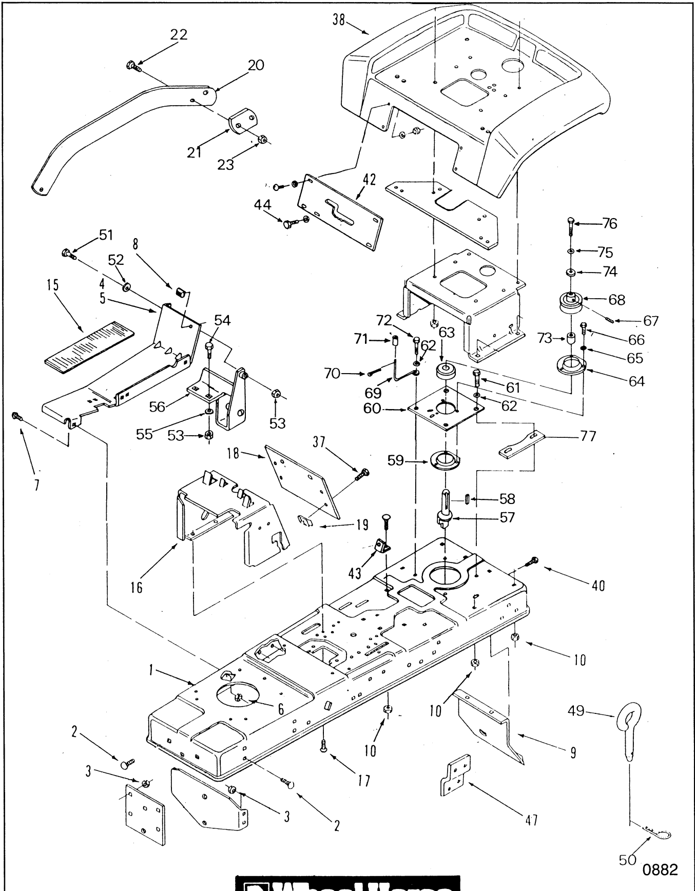
Figure 5-2 Frame, Sheet Metal and Covers
