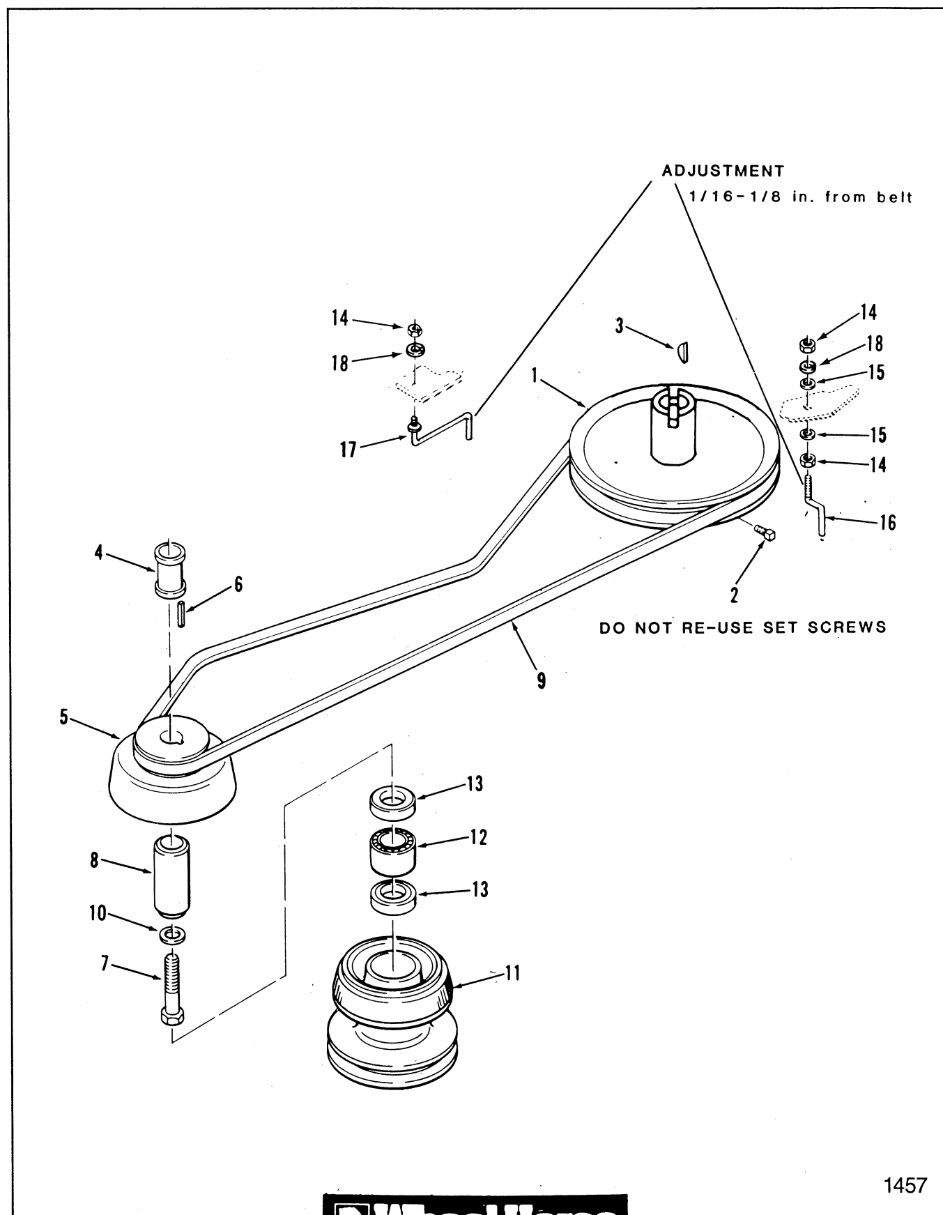
Figure 9-1 Drive Belt and Pulleys
