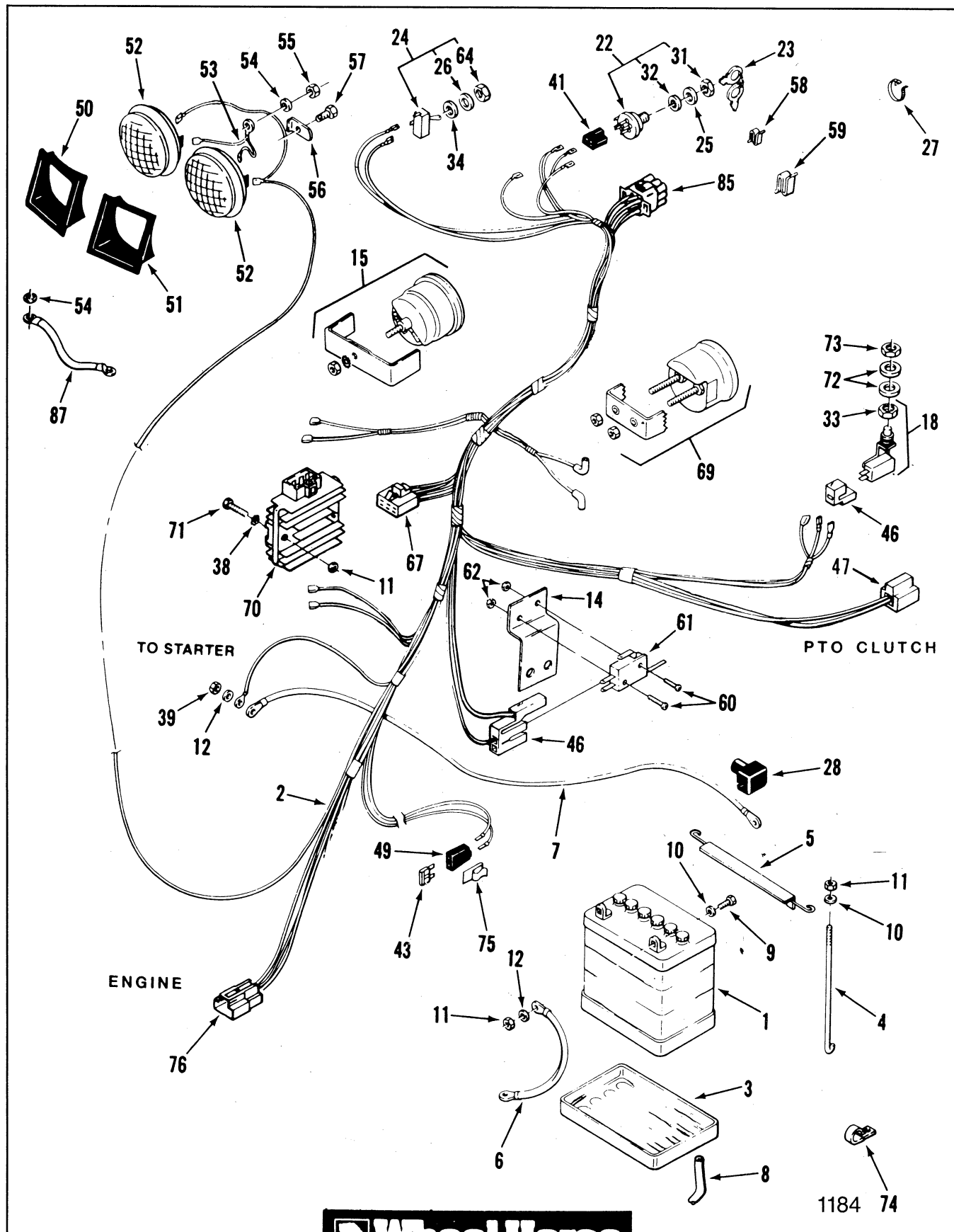
Figure 7-1 Electrical System
