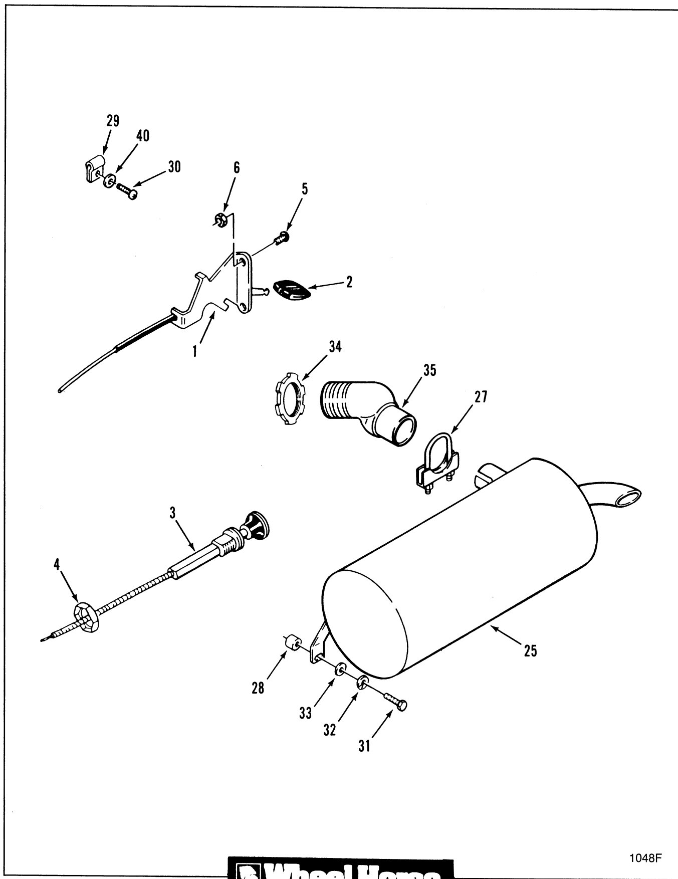
Figure 8-6 Throttle, Choke &amp; Exhaust
