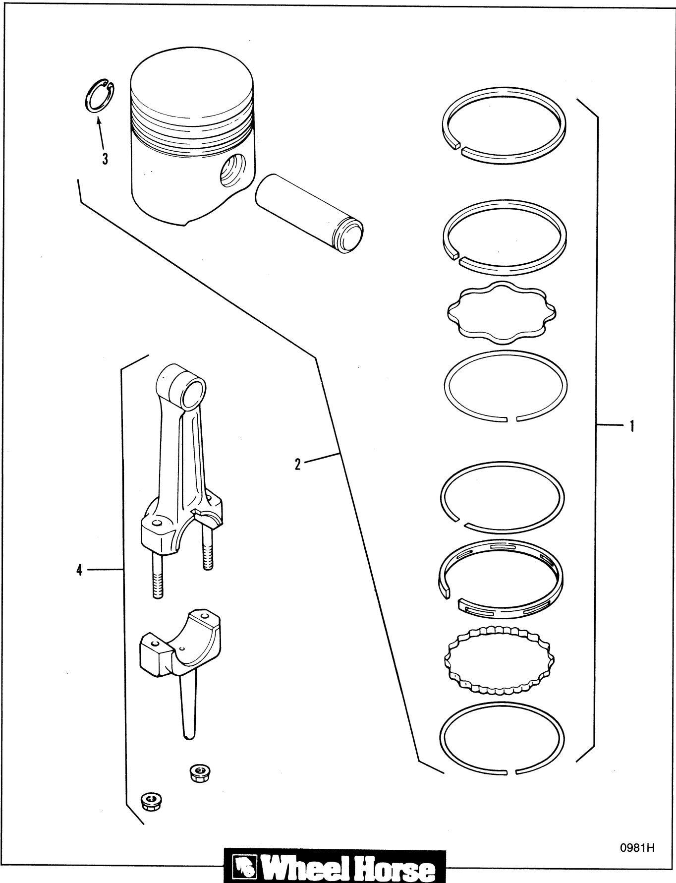
Figure 7-9 Piston &amp; Rings
