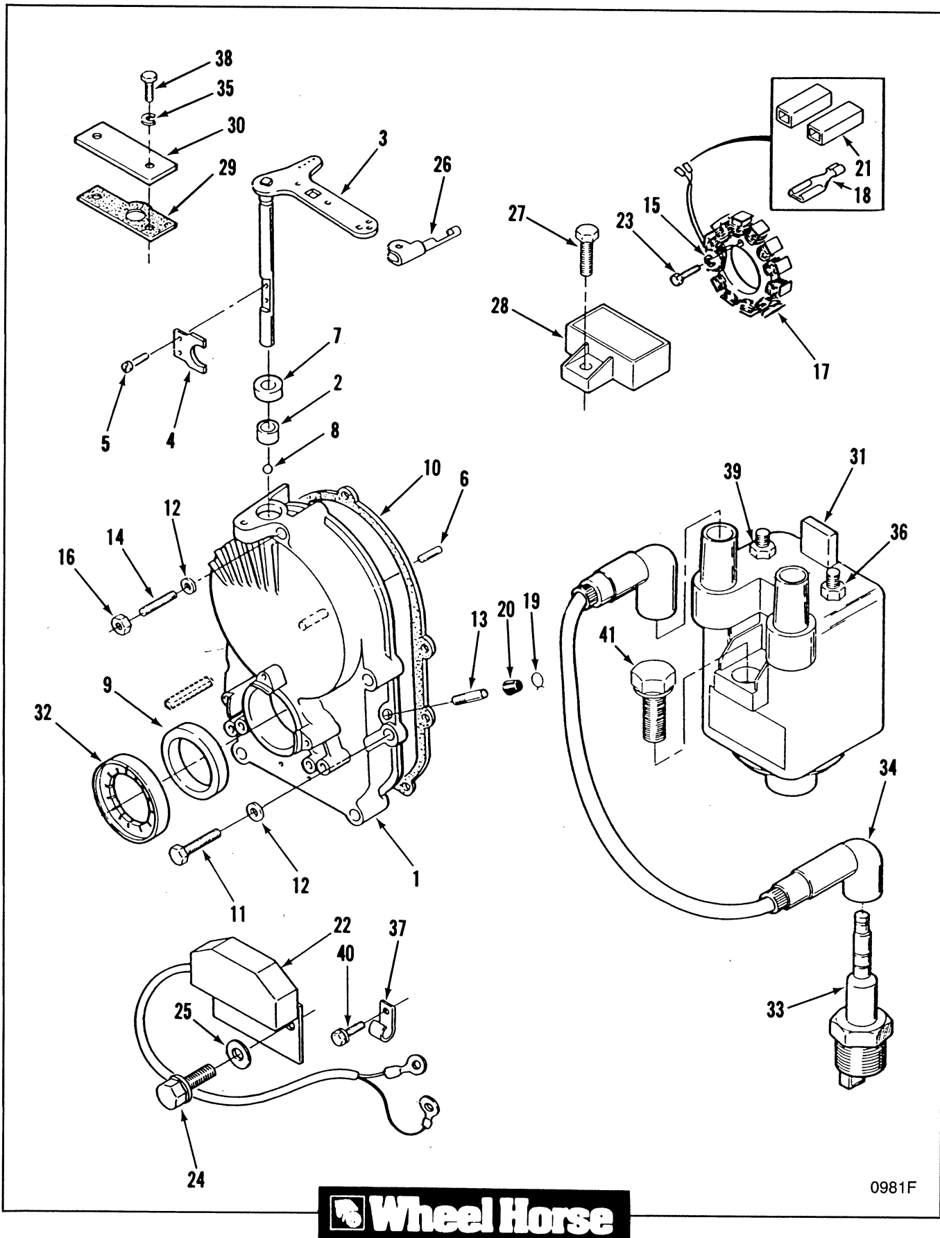
Figure 7-14 Onan Gearcase and Ignition Controls
