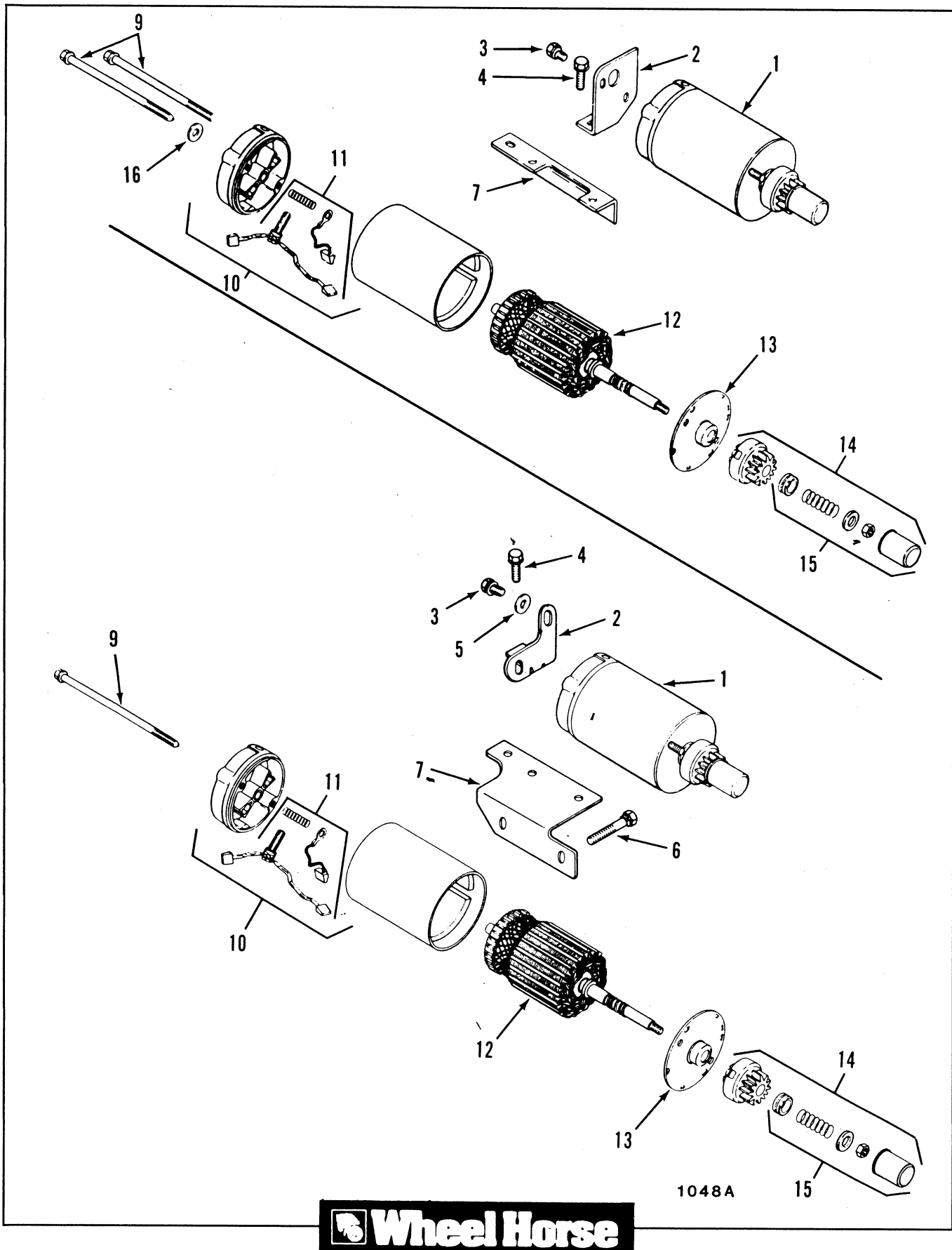
Figure 8-1 Starter
