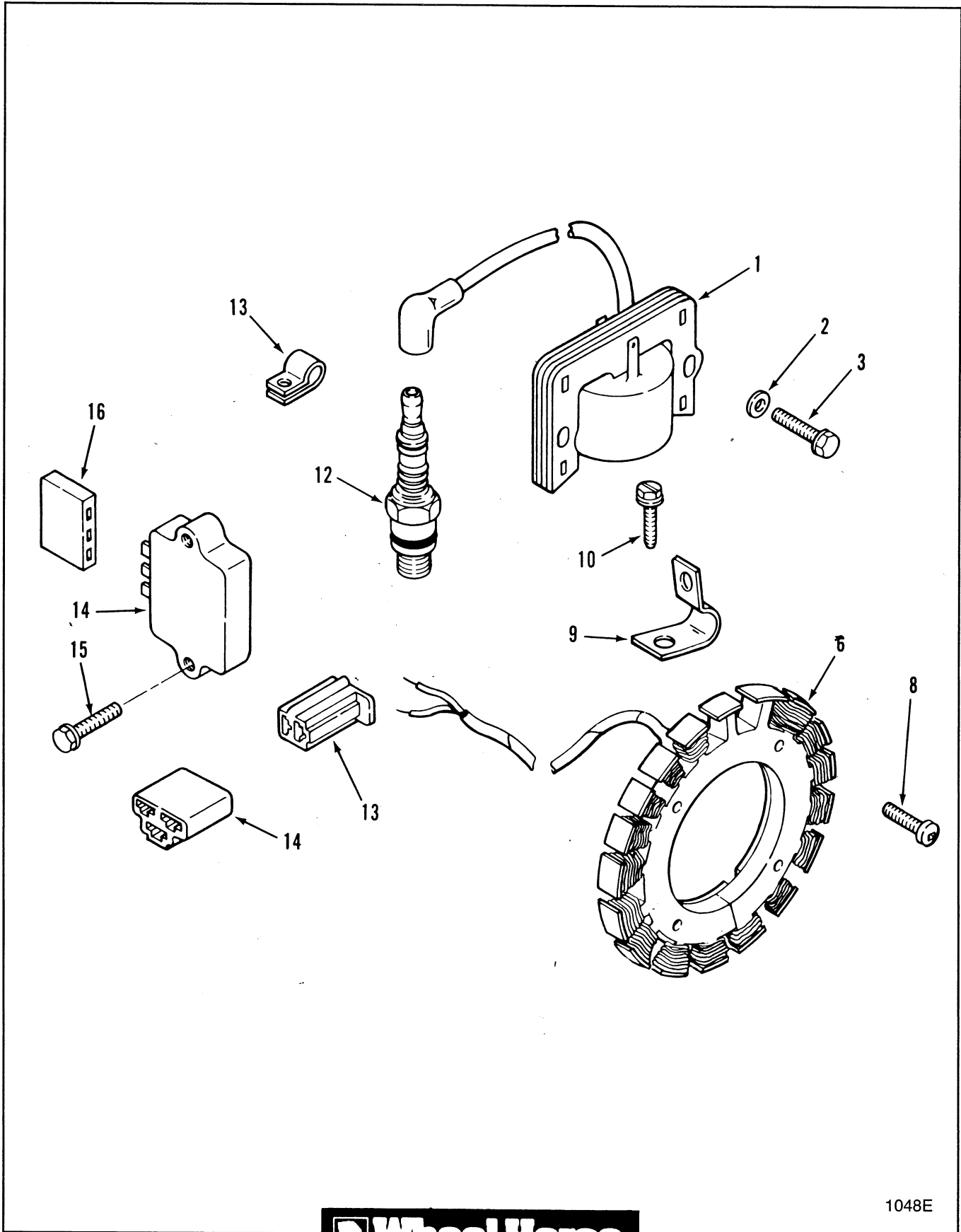
Figure 8-5 Ignition System
