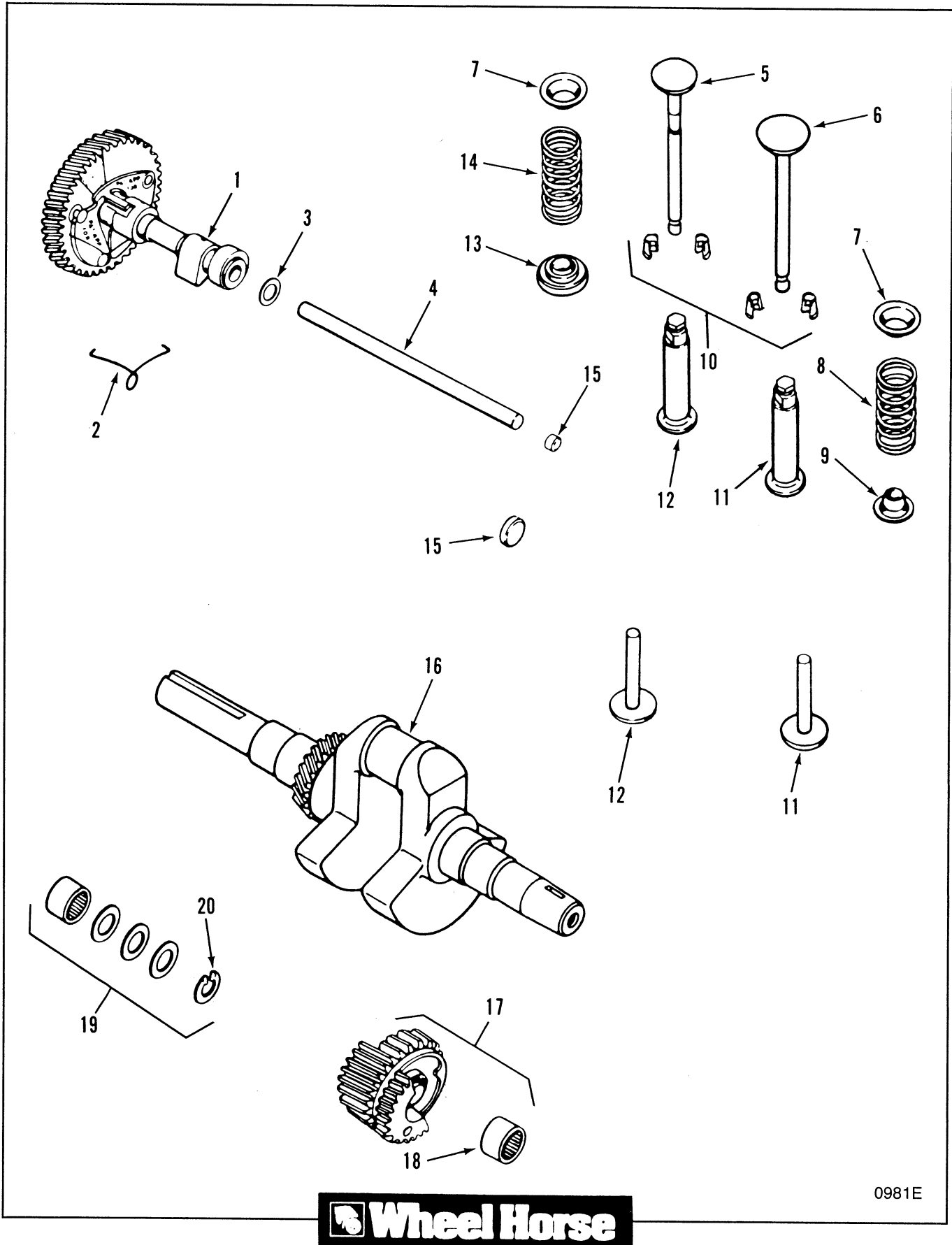
Figure 7-6 Camshaft, Crankshaft & Valves
