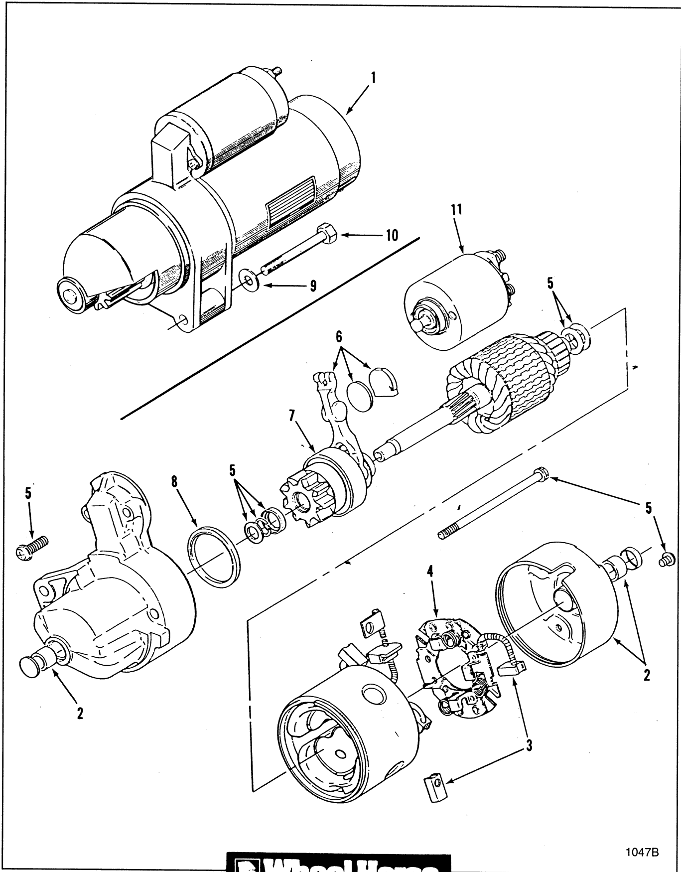
Figure 8-9 Onan Starter
