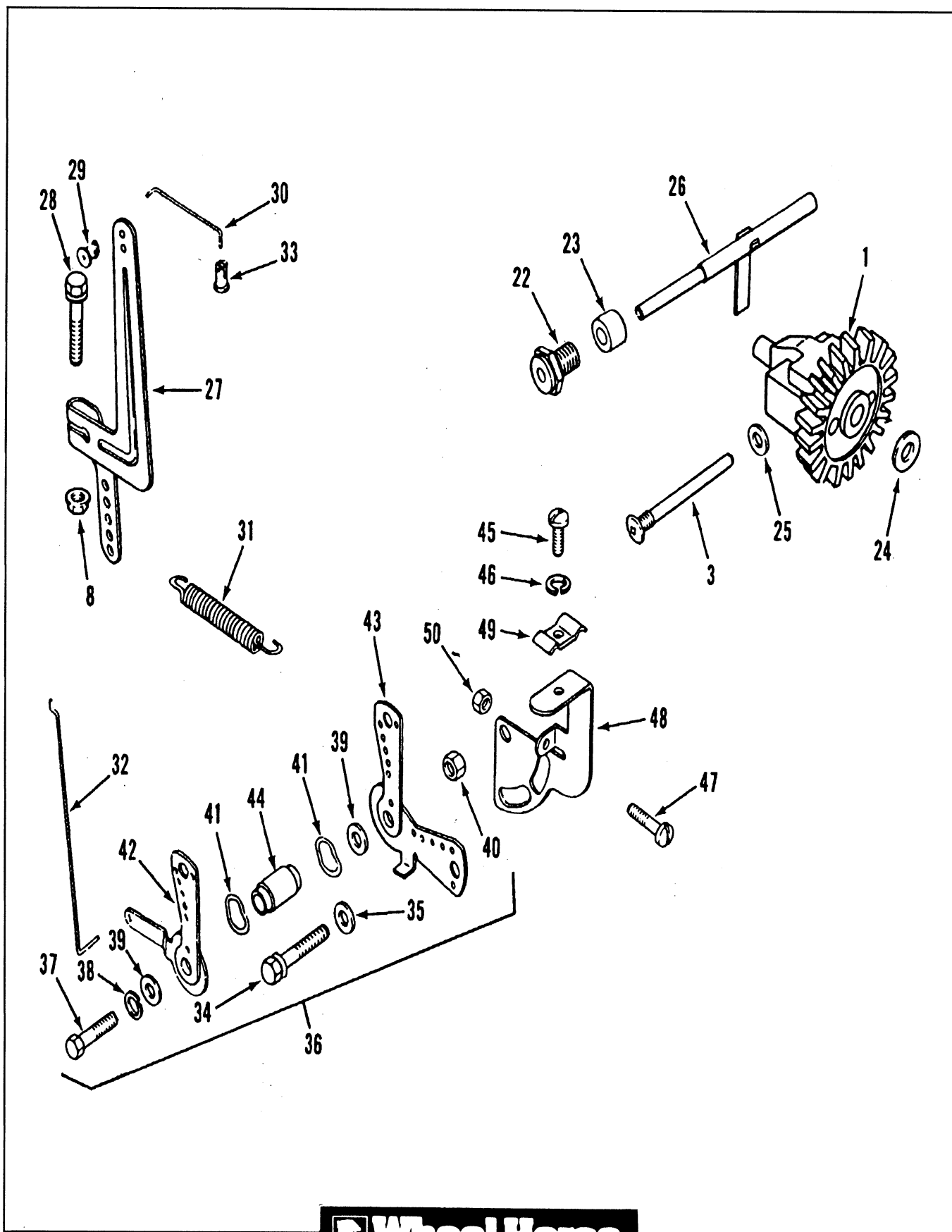
Figure 8-4 Governor Linkage
