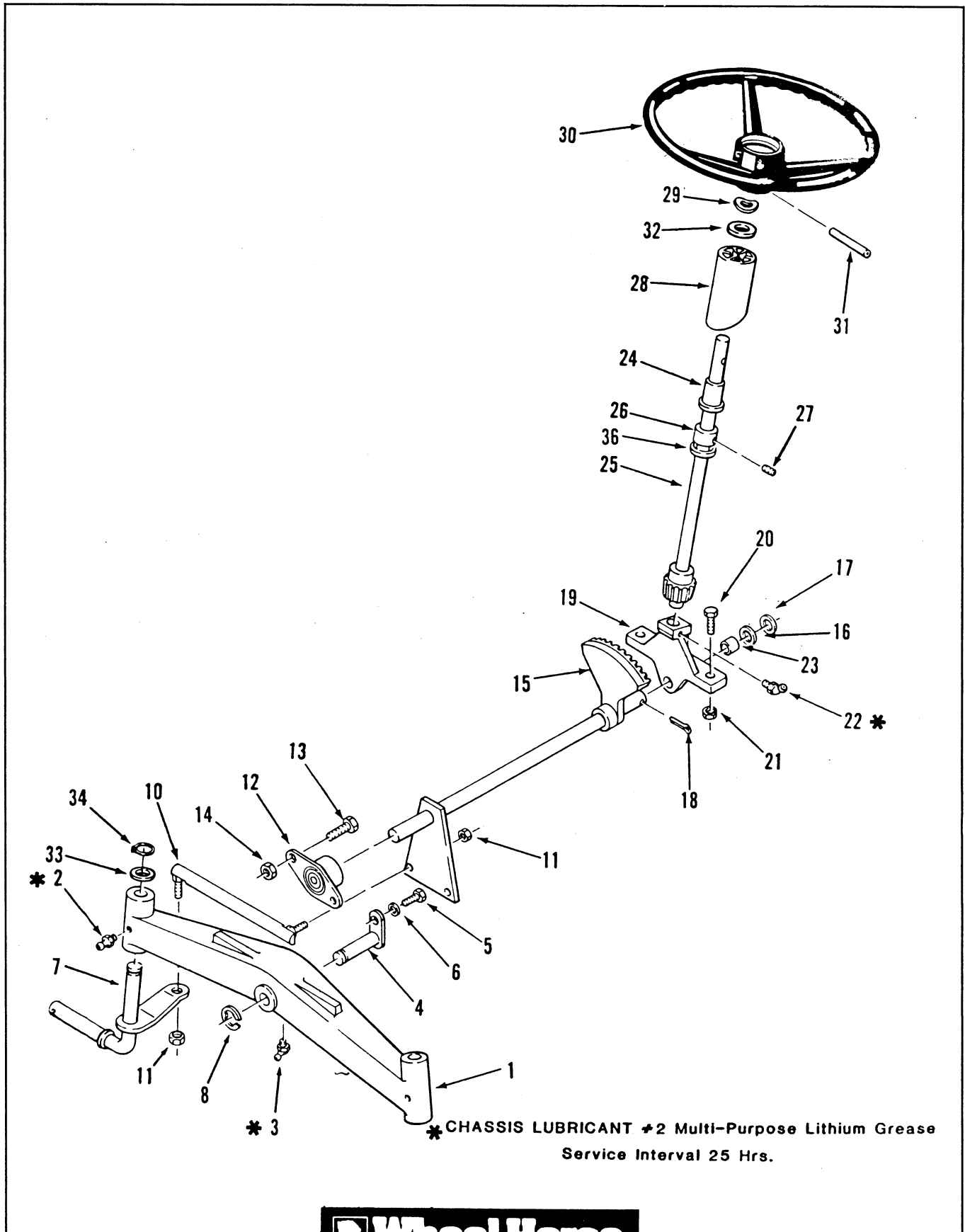
Figure 3 - 1 Front Axle and Steering
