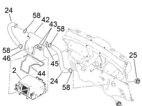
INTAKE AND AIR DUCT HOSE ASSEMBLY
