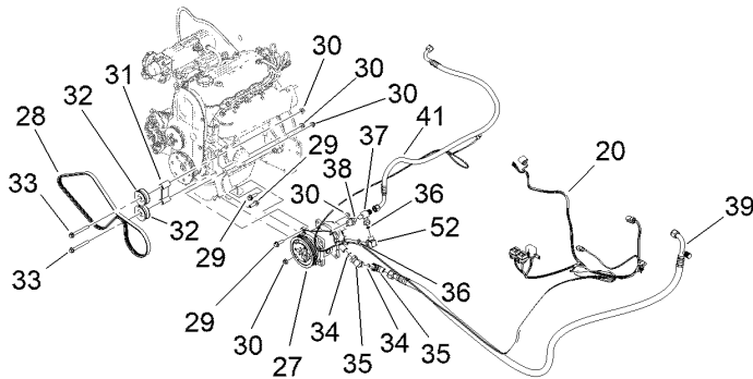
COMPRESSOR ASSEMBLY
