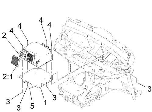
HVAC ASSEMBLY
