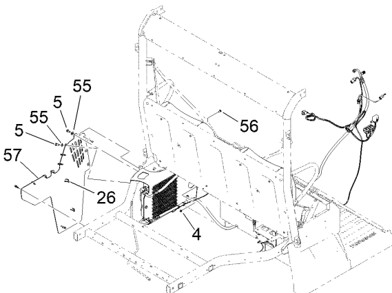
CONDENSER ASSEMBLY
