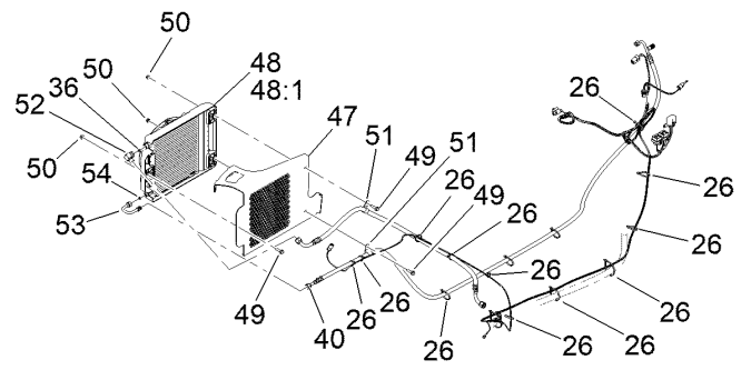
CONDENSER COMPONENT ASSEMBLY
