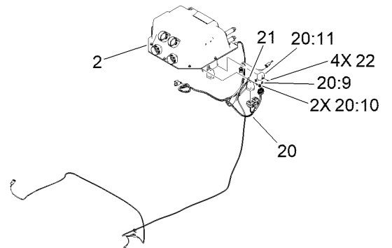
ELECTRICAL FUSES AND RELAYS ASSEMBLY
