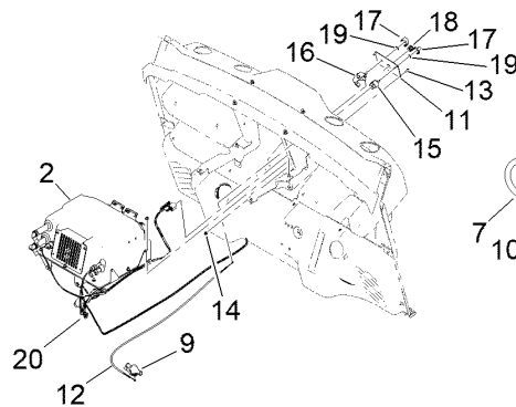
ELECTRICAL AND ROTARY CONTROL CABLE ASSEMBLY
