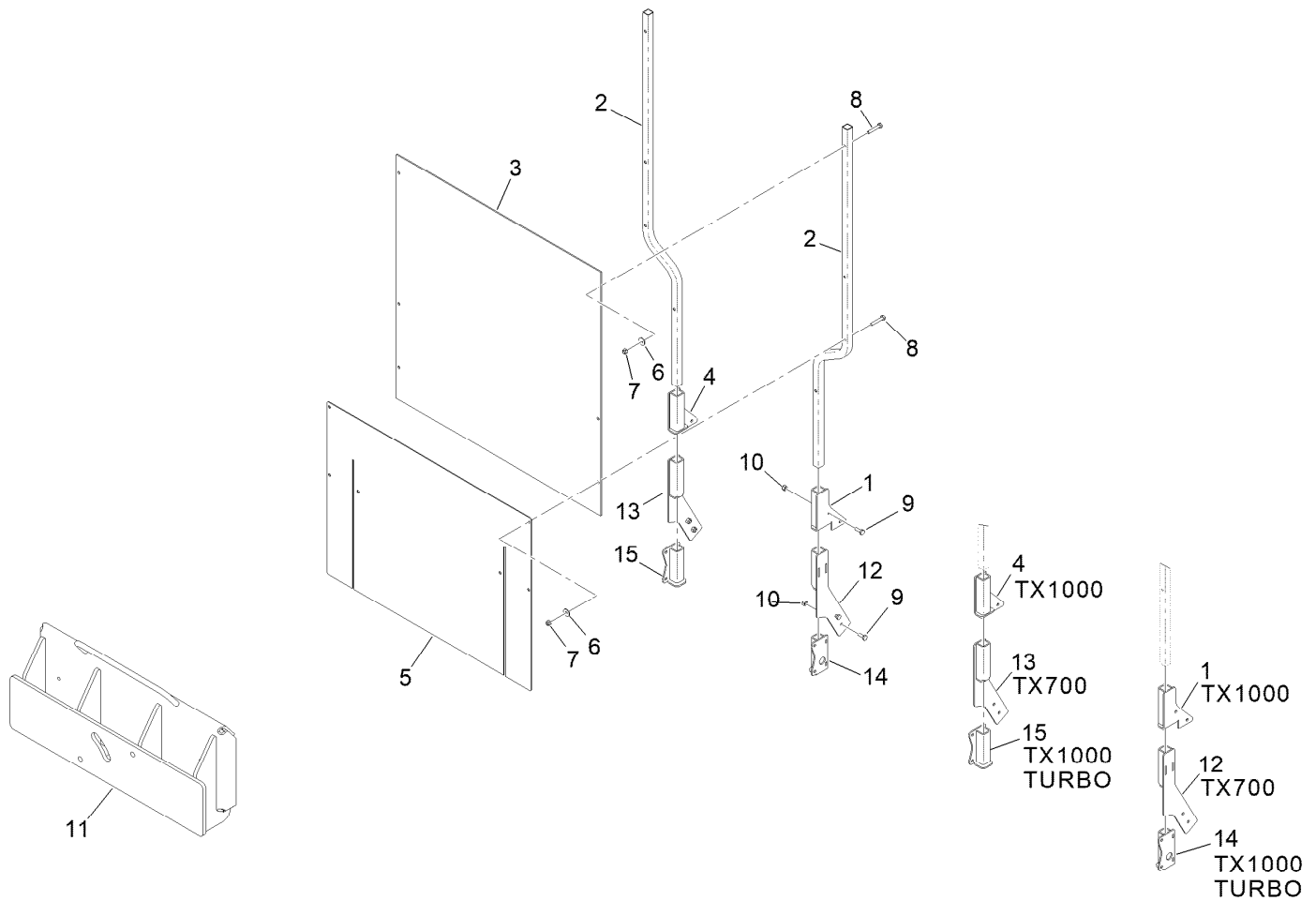
TX1000, TX700, AND TX1000 TURBO CONFIGURATION VIEW
