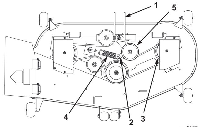
Figure 45 Top View
