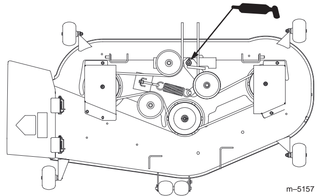
Figure 31 Top View
