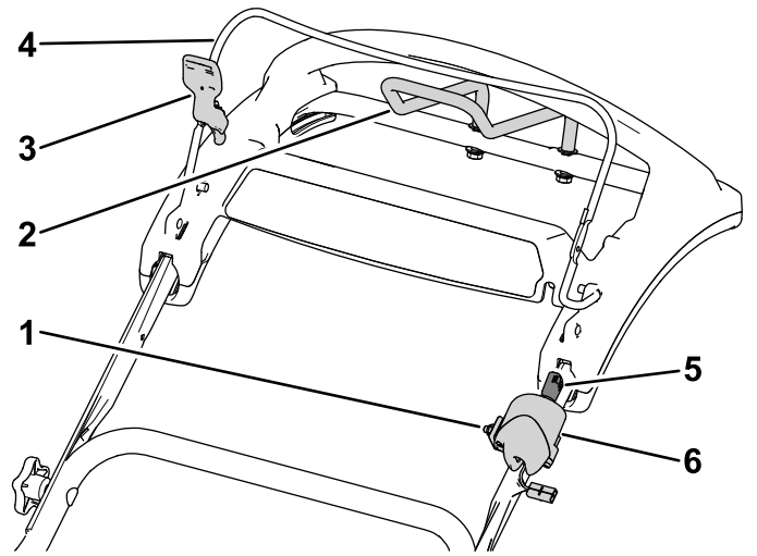
Figure 8 Upper handle
