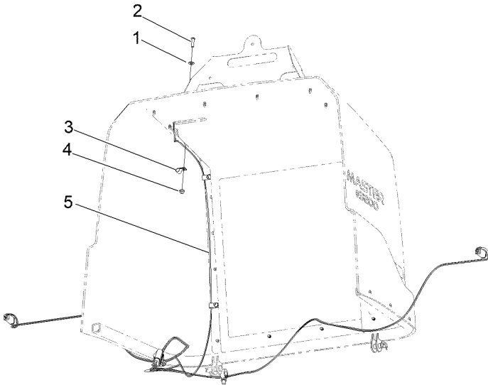
LICENSE PLATE LIGHT WIRE ROUTING
