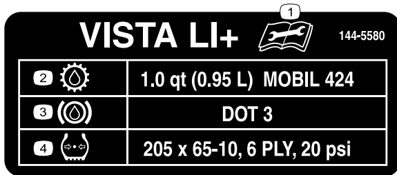
144-5580
