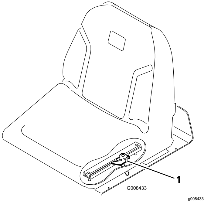
Figur 20
