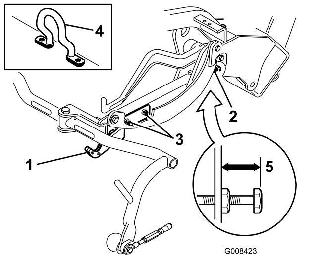
Figur 11
