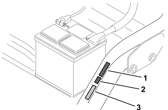
Figur 15
