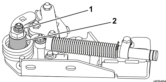
Figur 41
