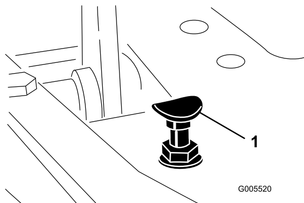
Figur 42
