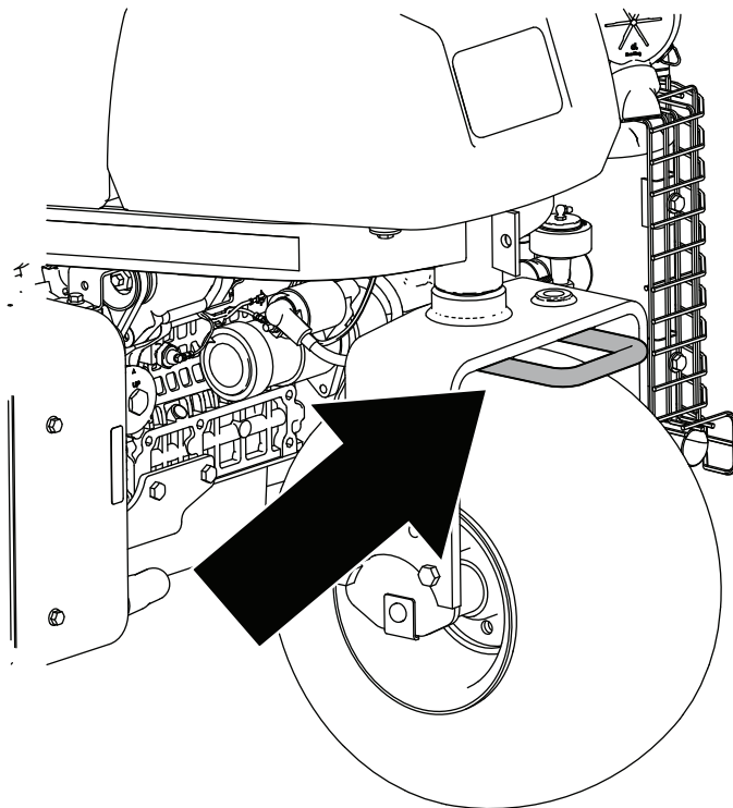
Figur 26
