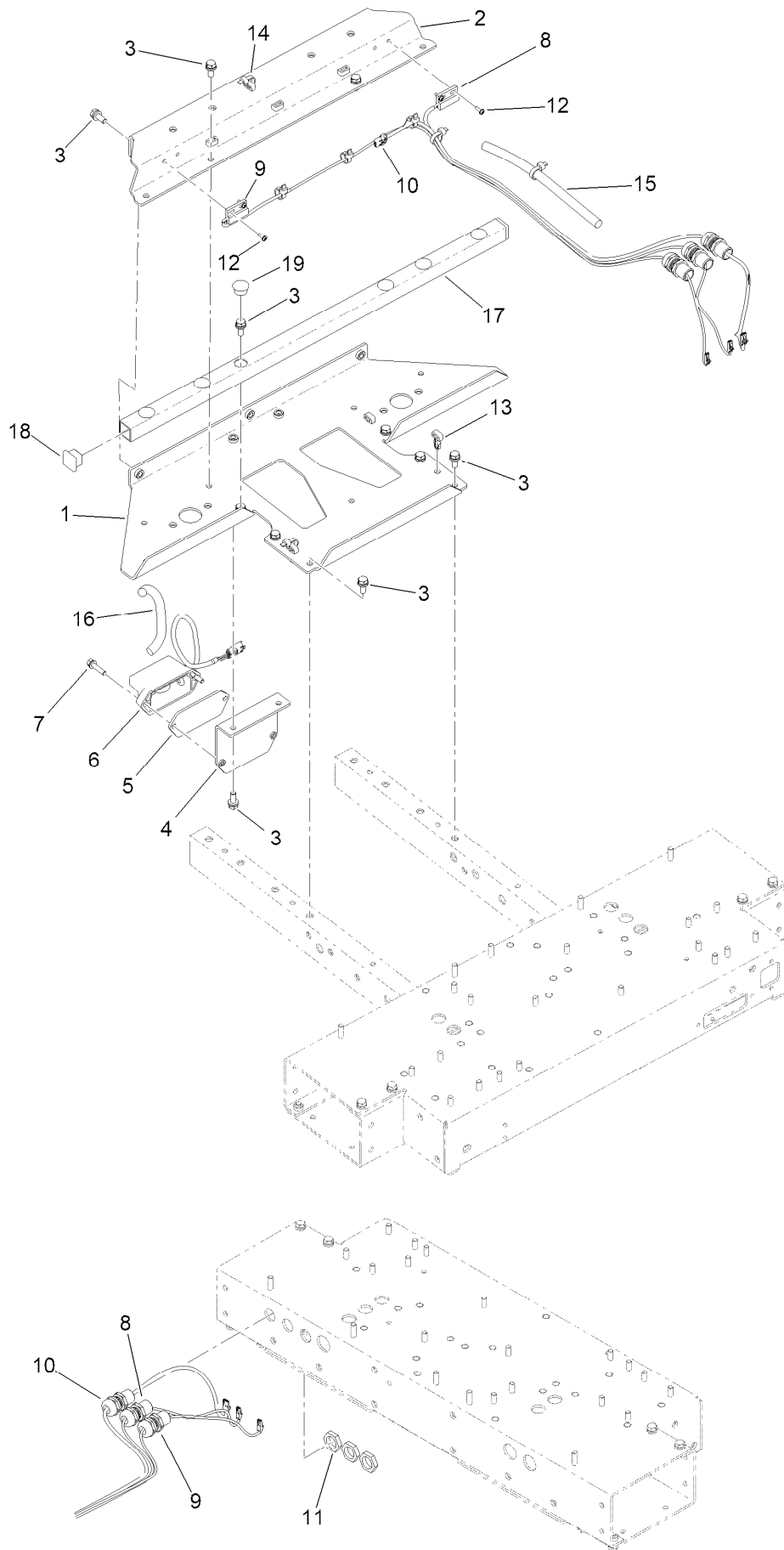
CABLE ASSEMBLY VIEW
