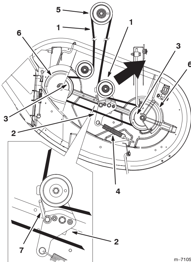
Figure 42 Top View
